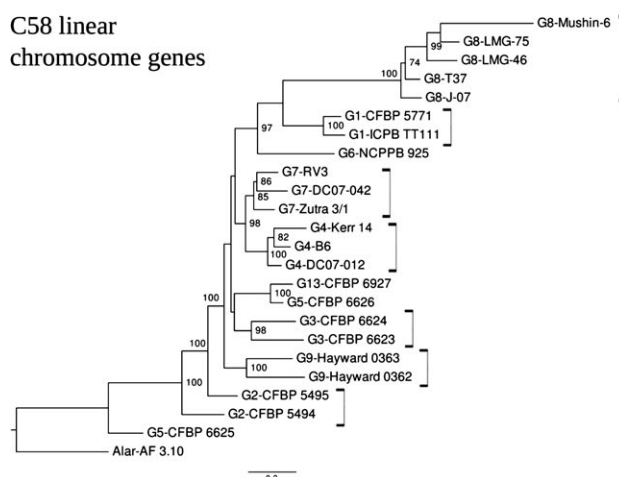
FIG. 2. —Clustering of Agrobacterium tumefaciens strains based on absence/presence of C58 CDS homologs. Neighbor-joining trees were constructed using the paralogous distances of Lake (1994) calculated from the presence/absence of C58 CDSs in other strains. With the reference genome being C58, this strain and its nearly identical relative DC07-004 were excluded from the analysis.
