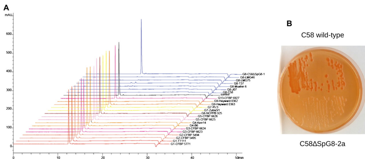
FIG. 5. —Experimental evidence of G8-specific phenotypes determined by SpG8 loci. (A) Ferulic acid degradation by A. tumefaciens strains determined by HPLC and UV spectrum at 320 nm. mAU, milli absorbance units. All genomovar G8 members were able to catabolize all ferulic acid in 12 h, contrary to non-G8 strains lacking SpG8-1b. (B) Curdlian production revealed by red dye on Congo red medium. C58: Agrobacterium tumefaciens wild-type strain C58 (red colonies), C58ΔSpG8-2a: SpG8-2a-deleted mutant (white colonies).
