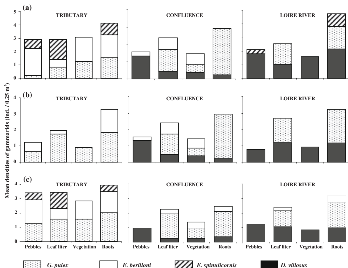
Fig. 1 Mean cumulative amphipod densities (individuals per 0.25 m²) at the microhabitat scale in a the Beuvron River, b the Cisse River and c the Thouet River. The first column represents sites in the tributary upstream from the confluence with the
