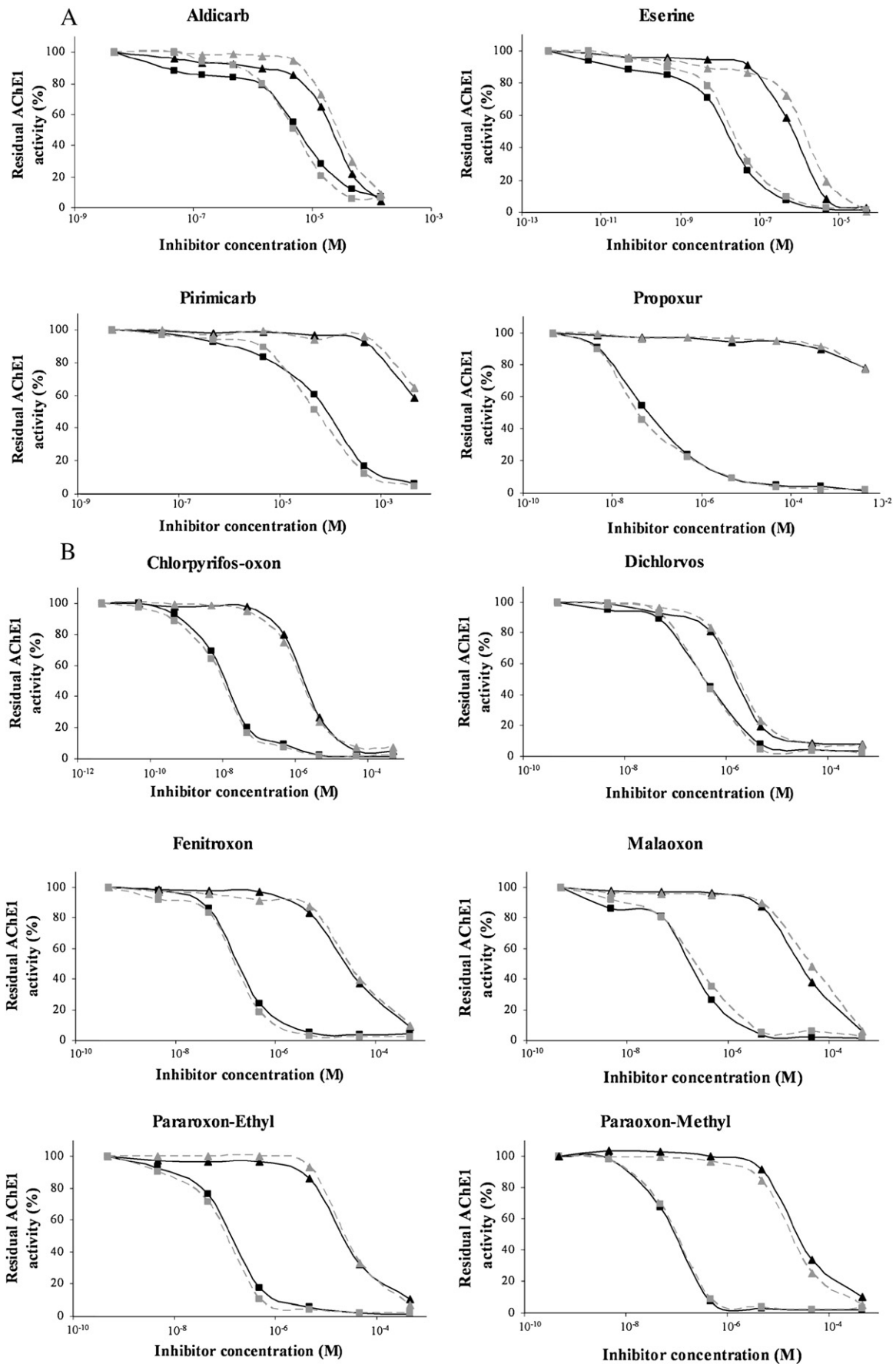
Fig. 2. Residual AChE1 activities of susceptible (squares) and resistant (triangles) mosquito head extract measured in presence of increasing dose of insecticides. Comparison between An. gambiae (black symbols) and C. pipiens (grey symbols) AChE1. (A) Carbamate insecticides; (B) Organophosphate insecticides.
