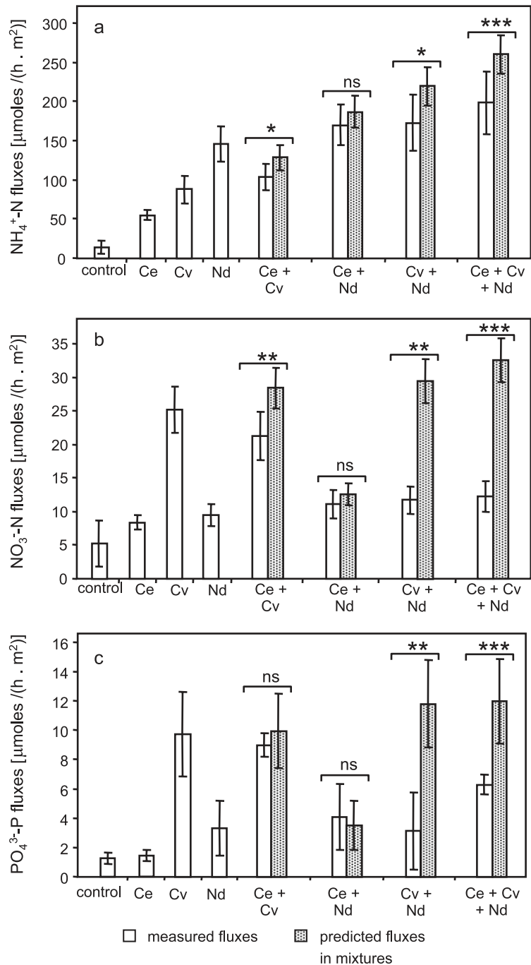
Fig. 4. Fluxes of ammonium (a), nitrate (b), and phosphate (c) across the water–sediment interface for the eight treatments. Rates are given as mean \pm S.D. of three cores. Predicted fluxes are indicated for the mixture treatments. The results of the statistical comparison between observed and predicted values are indicated on the graphs (*** p <0.001, ** p <0.01, * p <0.05, ns: no significant difference). Abbreviations of animal treatments are as in Fig. 2.
