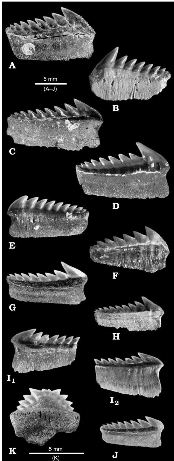
Fig. 3. Fossil Hexanchus sp. lower teeth from the Donzacq Formation of Saint-Géours-d'Auribat (late Ypresian/early Lutetian, south-western France). A. UMC-SG13, antero-lateral file, labial view. B. UMC-SG130, antero-lateral file, lingual view. C. UMC-SG15, lateral file, labial view. D. UMC-SG14, antero-lateral file, labial view. E. UMC-SG131, lateral file, lingual view. F. UMC-SG132, antero-lateral file, lingual view. G. UMC-SG17, lateral file, labial view. H. UMC-SG133, lateral file, labial view. I. UMC-SG134, broken lateral lower tooth with peculiar deep root, labial ( I 1 ) and lingual ( I 2 ) views. J. UMC-SG135, lateral file, labial view. K. UMC-SG12, symphyseal file, lingual view.
