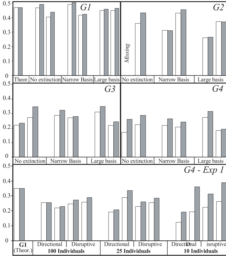
Figure 3. Estimates of gene diversity during the first four generations of experiment 2 (G1 to G4) and at the fourth generation in experiment 1. Data are missing for the second generation in the no extinction treatment. \square Within-population diversity H_s ; \blacksquare Total diversity H_t ; Theor : theoretically expected at the first generation.
