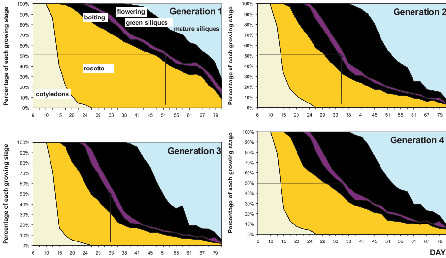
Figure 5. Evolution over time of the percentage of six growing stages (cotyledons, rosette, bolting, flowering, green pods and mature fruits) at the first generation (500 plants) and at the three subsequent generations (900 plants each, pooled over treatments).
