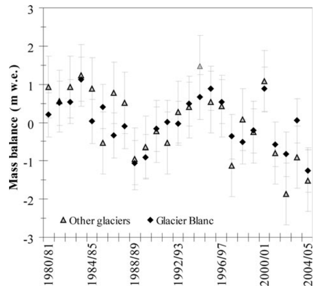
Fig. 5. Comparison of mass-balance series of French alpine glaciers. Glacier Blanc: black diamonds represent centred values computed by remote sensing and corrected with the CPDD method; vertical bars (black line) represent the 95% confidence interval. Other glaciers: triangles represent the average of the centred mass-balance series of five monitored glaciers in the French Alps (Argentière, Tacul, Gébroulaz, Saint-Sorlin and Sarennes); vertical bars (dashed line) represent the 95% confidence interval.
