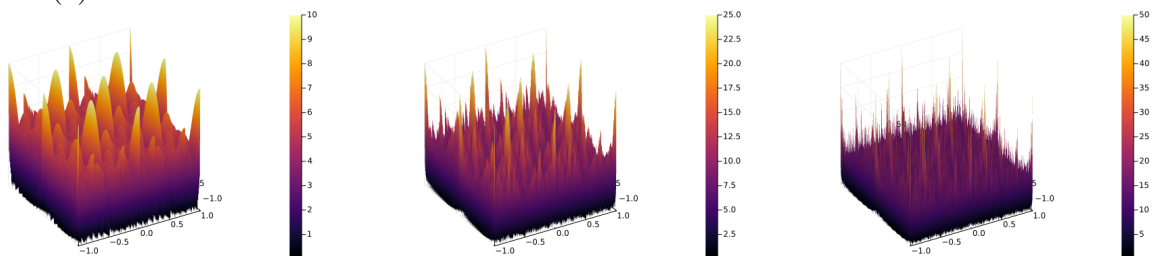
Figure: Plot of magnitude of Weyl sum for P(n) = ax^2 + bx with -0.001 \leq a, b \leq 0.001 , N = 10, 20, 50 .
