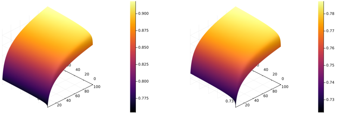
Figure: Plots of bound from Theorem 2.1 over bound from Proposition 2.19 for N = 300 , (in order)
