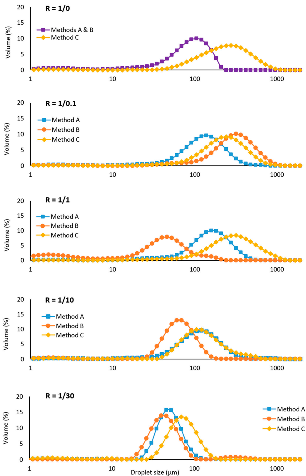
Figure 5. Droplet size distribution (volume-based) of Pickering emulsions stabilized by zein/tannic acid particles or aqueous solutions prepared by the different methods (A–C), at various zein/tannic acid molar ratios R from 1/0 (zein only) to 1/30. Emulsions were analyzed by laser diffraction directly after preparation, and the droplet size is plotted on a logarithmic scale.
