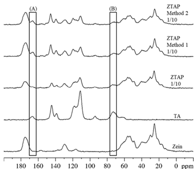
Figure 3. ^{13}\text{C} CP-MAS NMR spectra of tannic acid (TA), zein, zein–tannic acid physical mixture (ZTAP 1/10), zein–tannic acid particles prepared by method 1 (ZTAP method 1 1/10) and method 2 (ZTAP method 2 1/10). The peak labeled A appears at 166 ppm and the one labeled B at 73 ppm.
