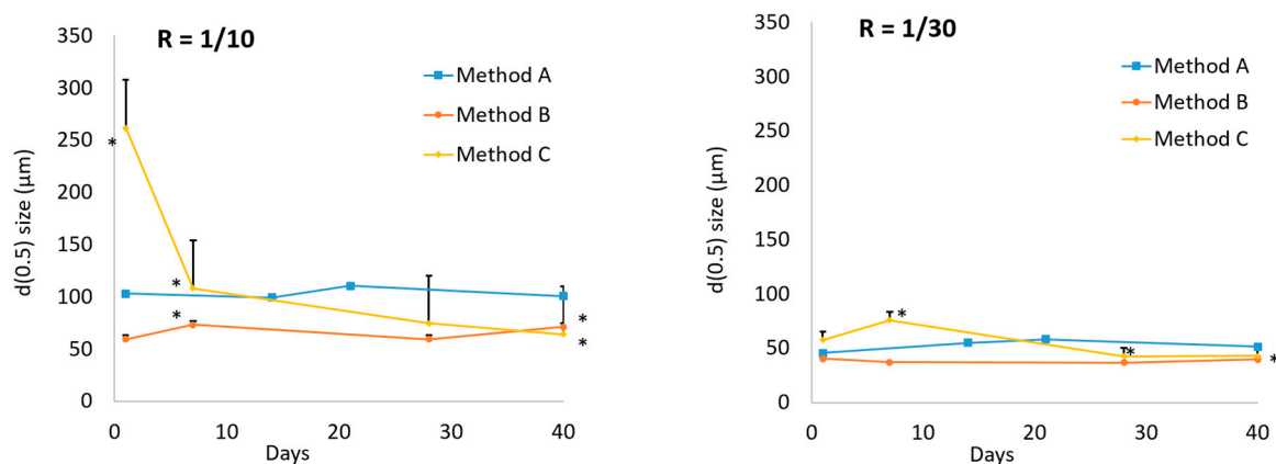
Figure 6. Stability of Pickering emulsions over time, assessed by monitoring the median droplet diameter ( D(0.5) ) over a 40-day period. Emulsions were prepared using different methods at zein/TA molar ratios of 1/10 and 1/30. Data are presented as mean \pm standard deviation ( n = 3 ). Statistical comparisons were performed using one-way ANOVA followed by Dunnett's post hoc test, * = p < 0.05 versus Day 1.
