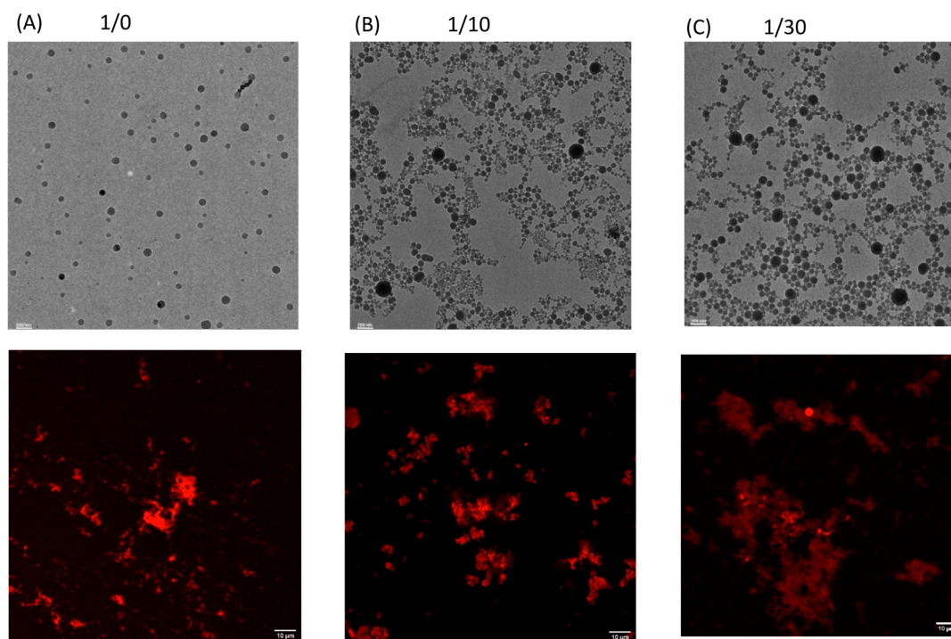
Figure 2. Images of particles prepared with method 1. (A) Zein particles alone. (B) ZTAP 1/10 and (C) ZTAP 1/30. The top rows of each ratio show transmission electron microscopy (TEM) images; the bottom rows show corresponding confocal laser scanning microscopy (CLSM) images. Scale bars: 200 nm (upper panels) and 10 \mu\text{m} (lower panels).
