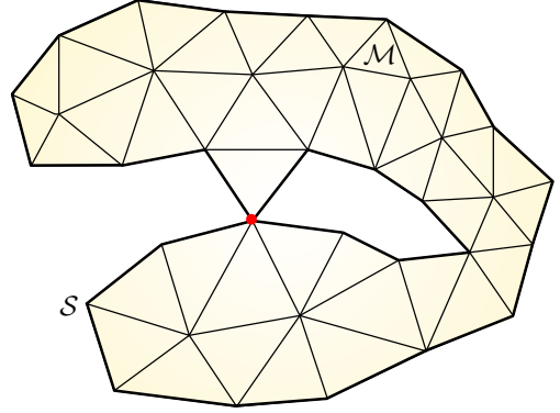
(B) A 2d mesh \mathcal{M} whose boundary mesh \mathcal{S} is the bold line: \mathcal{M} is non regular, since the region of the red boundary vertex is not homeomorphic to a half-plane.
