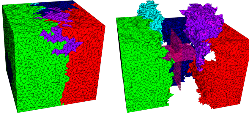
FIGURE 7. Partition of the cubic mesh containing the multi-screen geometry by partitioning directly \mathcal{M} with Algorithm 1, rather than its envelope \mathcal{M}^c .
