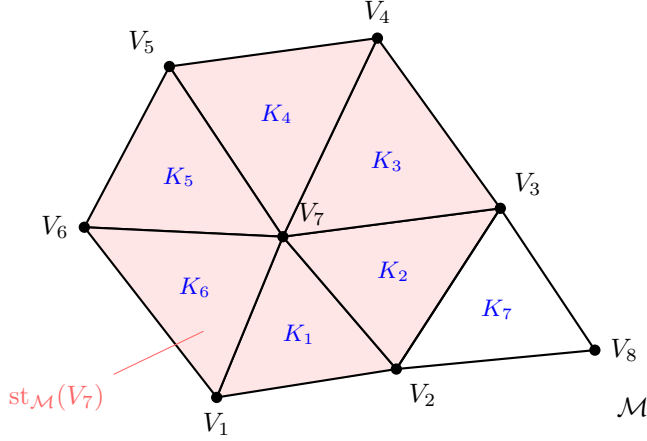
(A) A 2d simplicial mesh \mathcal{M} with vertices \{V_i\}_{1 \leq i \leq 8} and elements \{K_i\}_{1 \leq i \leq 7} . The star \text{st}_{\mathcal{M}}(V_7) of the vertex V_7 is made of the pink elements.
