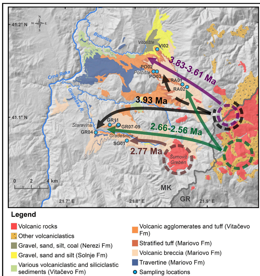
Fig. 8. Timing of the volcanic eruptions and interpreted source areas for Mariovo basin volcanoclastics.
