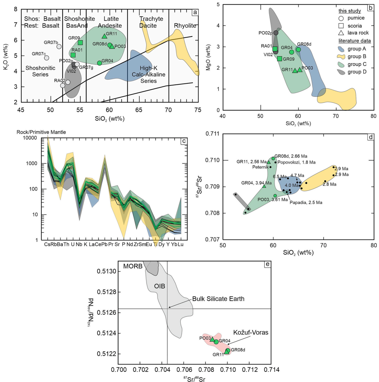
Fig. 6. Whole rock geochemical data of the studied samples compared to previously published results from the Kožuf-Voras volcanic system (summarized in Molnár et al., 2022). The groups A (blue), B (yellow), C (green) and D (grey) are updated from the hierarchical cluster analyses (Molnár et al., 2022). a: \text{SiO}_2 (wt%) vs. \text{K}_2\text{O} (wt%) modified after Peccerillo and Taylor (1976), where the pale grey circles indicate altered samples (not included in the other diagrams). b: \text{SiO}_2 (wt%) vs. \text{MgO} (wt%). c: trace element diagram normalized to primitive mantle (Sun and McDonough, 1989). d: ^{87}\text{Sr}/^{86}\text{Sr} ratio vs. \text{SiO}_2 (wt%) with ages from literature data and names of the relevant lava domes presented. e: ^{87}\text{Sr}/^{86}\text{Sr} vs. ^{143}\text{Nd}/^{144}\text{Nd} ratios (Bulk Silicate Earth value, MORB and OIB fields are from Zindler and Hart, 1986). (For interpretation of the references to colour in this figure legend, the reader is referred to the web version of this article.)
