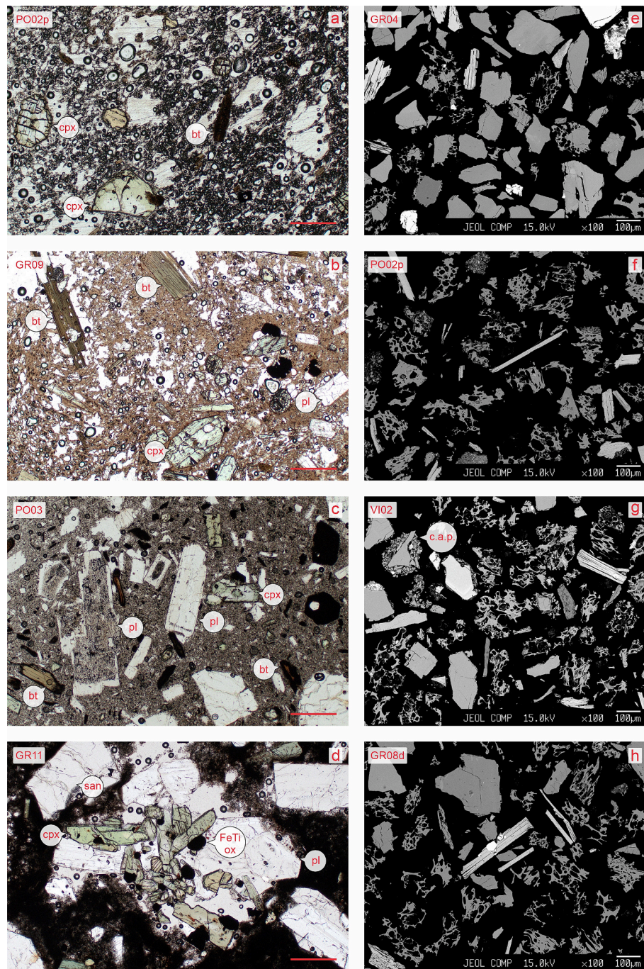
Fig. 5. Petrographic microscopic photos (1 N) of selected pumice (a), scoria (b) and lava rock samples (c-d); and BSE images of selected pumice samples (e-h; 125–250 \mu\text{m} fraction). The scale is 500 \mu\text{m} unless otherwise marked. Complex zonation of clinopyroxene (a, c), sieved plagioclase (c) and mafic crystal agglomerate (d) are characteristic of the samples. cpx: clinopyroxene, bt: biotite, pl: plagioclase, san: sanidine, Fe—Ti ox: Fe—Ti oxide, c.a.p: cored ash pellet.
