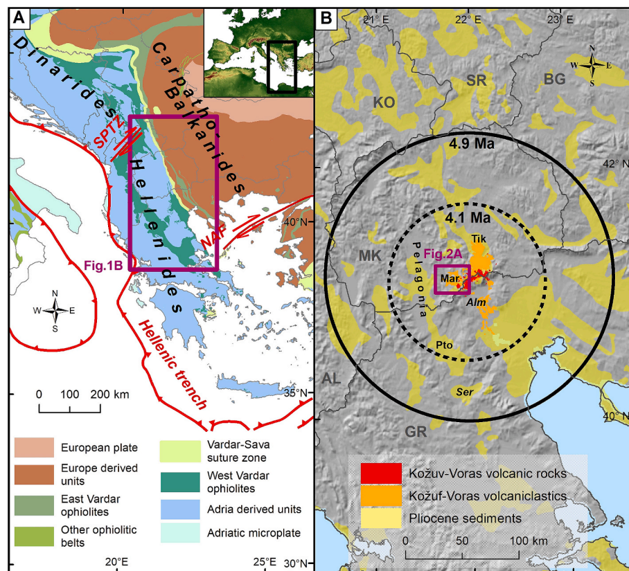
Fig. 1. Location of the study area. A: Geotectonic setting of SE Europe (modified after Schmid et al., 2020). SPTZ: Skutari-Peč transverse zone, NAF: North Anatolian Fault. B: Location of the Kožuf-Voras volcanic system in relation to basins with Pliocene sediments in the central parts of SE Europe. Estimated dispersal ranges for the 4.9 Ma and 4.1 Ma eruptions are indicated (based on Vougioukalakis, 2002). Mar – Mariovo basin, Tik – Tikveš basin, Pto – Ptolemais basin, Ser – Serbia basin. Shaded relief based on digital elevation data from SRTM 1 Arc-Second Global dataset, https://doi.org/10.5066/F7PR7TFT .
