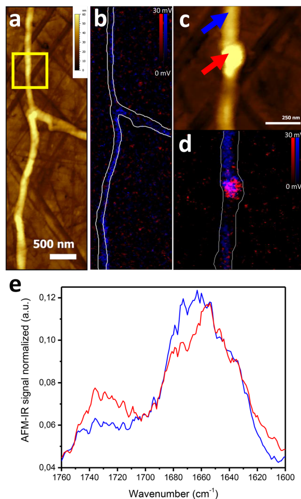
Fig. 4 Thermal alteration of a single collagen fibril. (a) AFM topography of the region prior to thermal treatment; (b) composite IR map showing absorbance at 1660\text{ cm}^{-1} (blue) and 1725\text{ cm}^{-1} (red) of the fibril before thermal treatment; (c) AFM topography acquired after thermal alteration, corresponding to the yellow square highlighted in panel (a); (d) composite IR map showing absorbance at 1660\text{ cm}^{-1} (blue) and 1725\text{ cm}^{-1} (red) of the fibril after thermal treatment (e) IR spectra recorded at the positions indicated by the colored arrows, showing a comparison between a non-heated region (blue) and the globular structure formed after localized heating (red).
