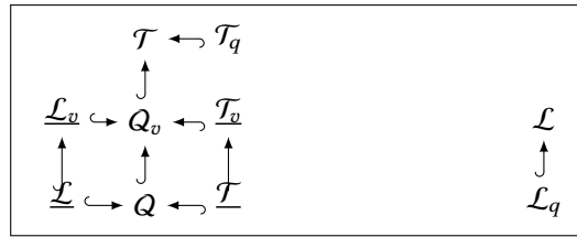
Fig. 1. Inclusion relationship ( \leftrightarrow ) between subsets of the set of terms \mathcal{T} and subset \mathcal{L}_q of \mathcal{L} .
