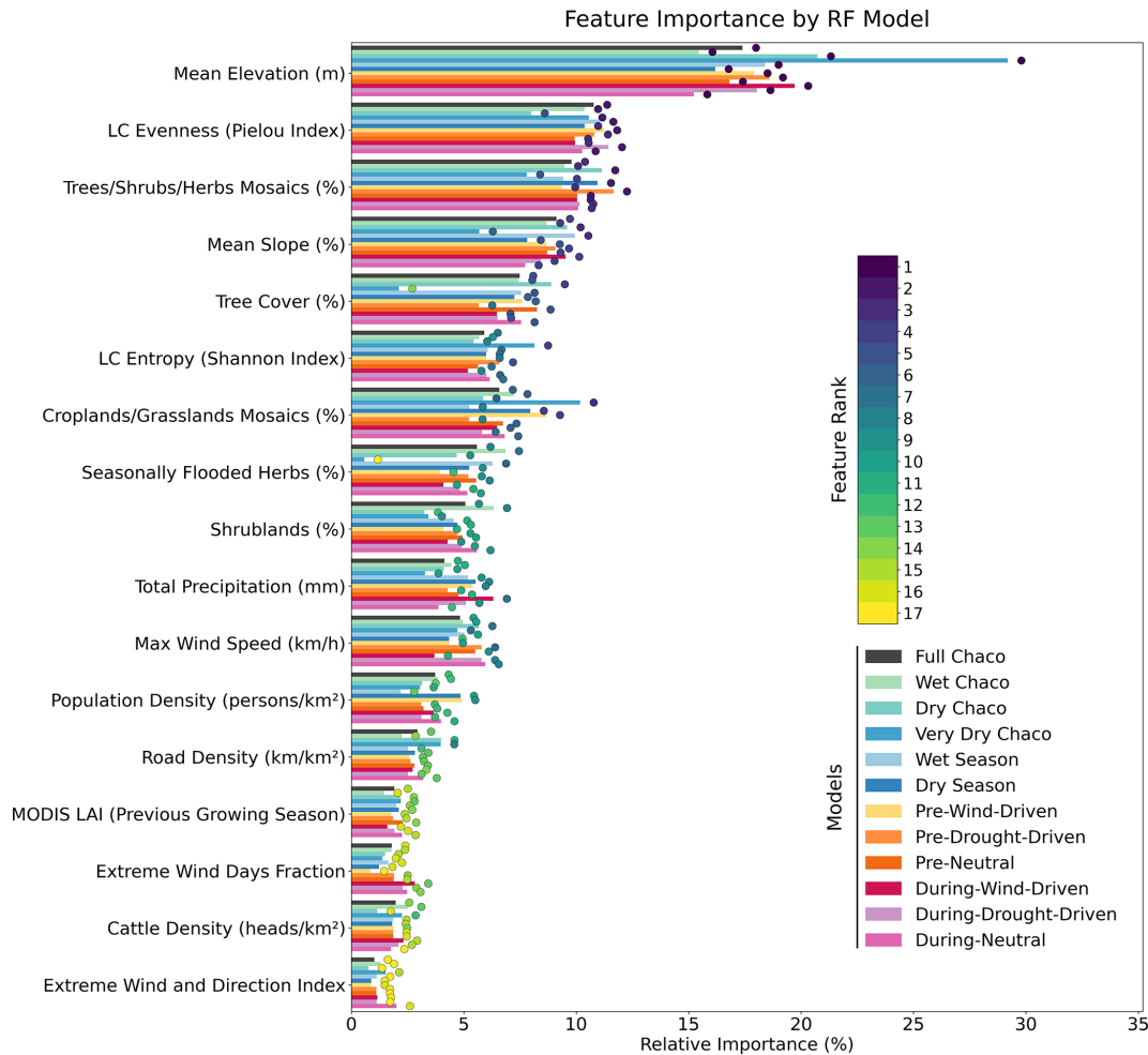
Figure 15. SHAP feature importance ranks across all trained Random Forest models used to predict fire patch size ( n_{cell} ) based on 17 explanatory variables. Colored dots at the end of bars shows the rank of a variable’s importance (1 = most important, 17 = least important) for a given model.
