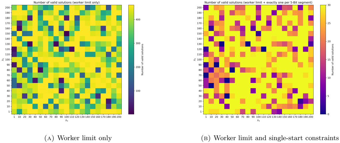
FIGURE 5. Number of valid solutions under single and combined constraints.
