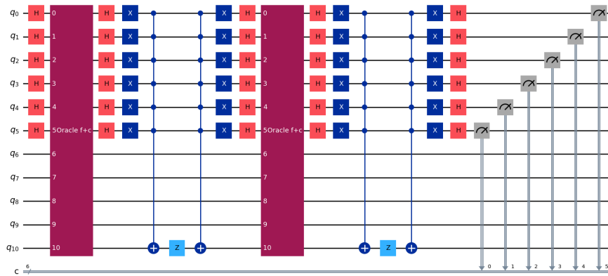
FIGURE 2. Quantum circuit using GAS for solving the toy example with two iterations.
