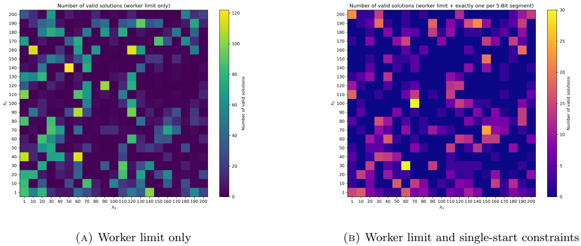
FIGURE 6. The number of valid solutions of the top 200 high-probability solutions under single and combined constraints.
