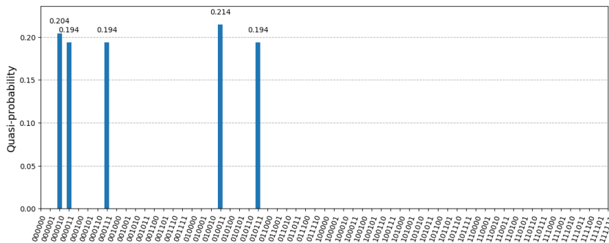
FIGURE 3. Probability of reaching a feasible solution
