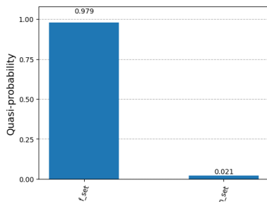
FIGURE 4. Probability of reaching a solution in the feasible solution set: f\_set is feasible set (that contains feasible solutions) and n\_set is non-feasible set.
