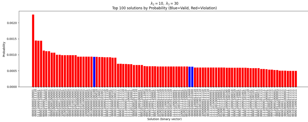
(A) Probabilities of the top 100 solutions found by QAOA. Blue bars indicate solutions meeting the worker limits; red bars indicate violations.
