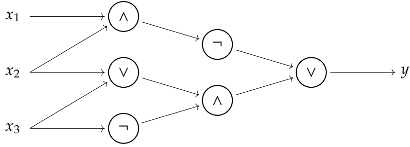
Figure 1: A Boolean circuit of size 6 and depth 3 with three inputs ( x_1, x_2, x_3 ) and one output. The gates are \wedge (AND), \vee (OR), and \neg (NOT). Truth assignment \tau = (1, 1, 1) evaluates to 0 (false), while assignment \tau' = (1, 1, 0) evaluates to 1 (true).
