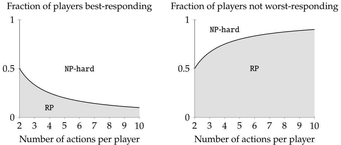
Figure 3: Schematic comparison of tractability frontier for best-responding and not worst-responding.
