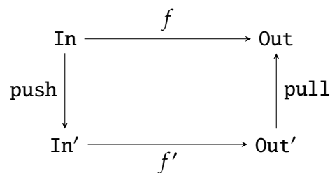
Figure 2: Reduction from f to f' .
