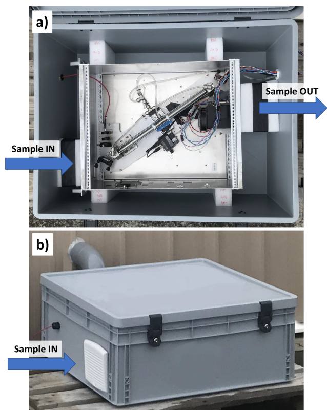
Figure 2. Pictures of the optical compartment. (a) View inside the plastic box. The internal rack has a cover that was removed for the picture. (b) The plastic box installed and ready for outdoor air measurements.
