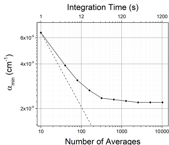
Figure 4. The minimum absorption coefficient \alpha_{\text{min}} versus the number of spectral averages for the OP-IBBCEAS instrument. For these measurements, the instrument was installed in a pristine location to test the instrument in background conditions where \text{NO}_2 concentrations during the measurement period were \sim 0.55 ppb. Absorption spectra were averaged for different integration times, and \alpha_{\text{min}} was calculated from the standard deviation of the residual.
