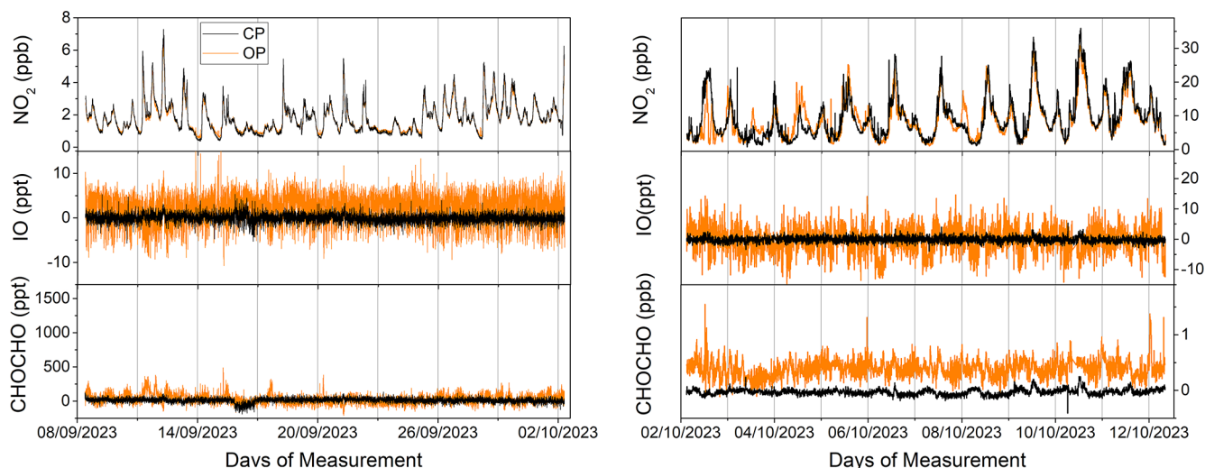
Figure 5. Left: 24 d comparison between close-path and open-path indoor air measurements using the two IBBCEAS instruments. The sample inlet of the close-path system was placed as close as possible to one of the open-path instruments. Mean values are -0.06 \pm 1.96 and 2.26 \pm 6.83 ppt for IO and -12.2 \pm 67 and 29.7 \pm 144 ppt ( 2\sigma ) for CHOCHO for the CP and OP system, respectively. Right: 10 d comparison between close-path and open-path outdoor measurements conducted in Grenoble using the two IBB-CEAS instruments. The sample inlet of the close-path system was placed close to the open-path instrument. Mean values are -0.09 \pm 1.78 and -0.29 \pm 8.8 ppt for the IO and -37.6 \pm 108 and 388 \pm 380 ppt ( 2\sigma ) for CHOCHO for the CP and OP system, respectively.
