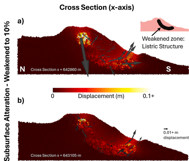
Fig. 11. We show the results of weakening a concave upward listric structure (reduction to 10% of the original bulk strength) within the subsurface that represents a region with high electrical conductivity values in Rosas-Carbajal et al. (2016). Panels (a) and (b) display parallel cross-sections positioned approximately at the western and eastern boundaries of the Bulge, respectively. This spacing (~200 m) captures the variability of deformation across the southern flank. Panel (a) corresponds to the western bound, while (b) corresponds to the eastern bound. Displacement vectors are normalised and limited to a maximum magnitude of 0.1 m (10 cm). For visualisation purposes, vector lengths are scaled by a factor of 500. Thus, a plotted arrow length of 500 units represents a real displacement of at least 0.1 m.
