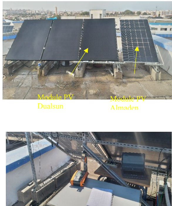
Fig. 2. PV modules and experimental setup for data acquisition.
