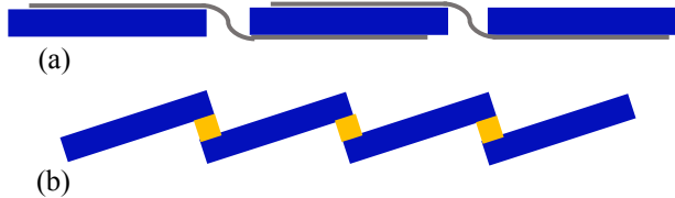
Fig. 1. schematic diagram of conventional copper ribbon interconnection (a) and shingle interconnection (b) for silicon solar cells.
