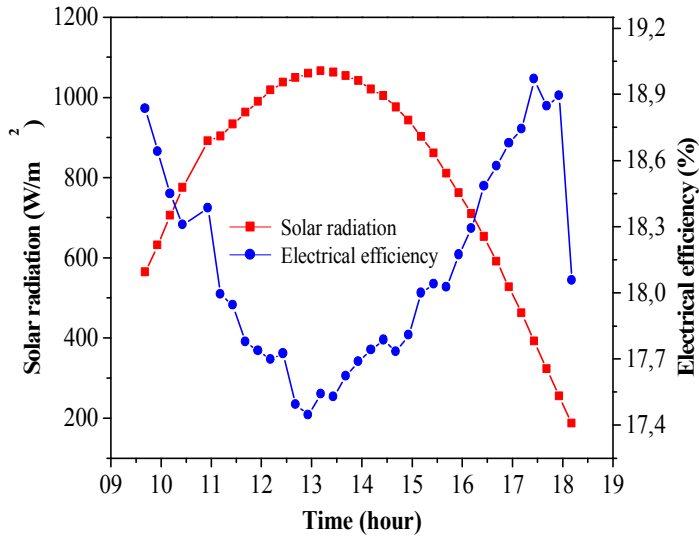
Fig. 5. Effect of solar irradiation on the electrical efficiency of the Dualsun PV module.
