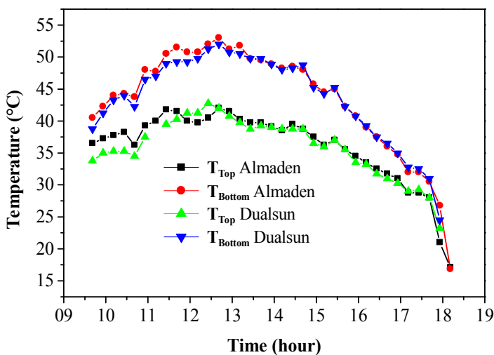
Fig. 8. Temperature evolution of the front and rear surfaces of PV modules.
