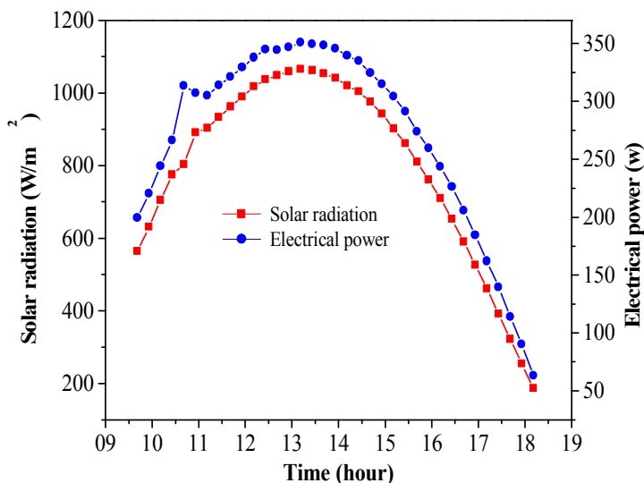
Fig. 4. Effect of solar irradiation on the electrical output of the Dualsun PV module.
