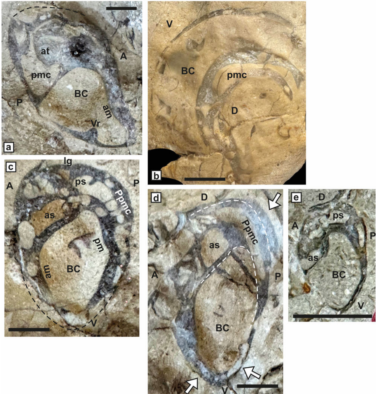
Figure 21: Pachytraga aff. paradoxa , Saint-Montan (JPMA 18071). a) Longitudinal oblique section of LV showing the myocardinal elements and the ventral inner ridge. b) Longitudinal section of a LV showing the arcuate habit. c) Transverse section of a RV showing the canaliculated architecture. d) Sections of RV focusing on canaliculation (arrows). e) Transverse apical /juvenile section. Scale bar 10 mm.
