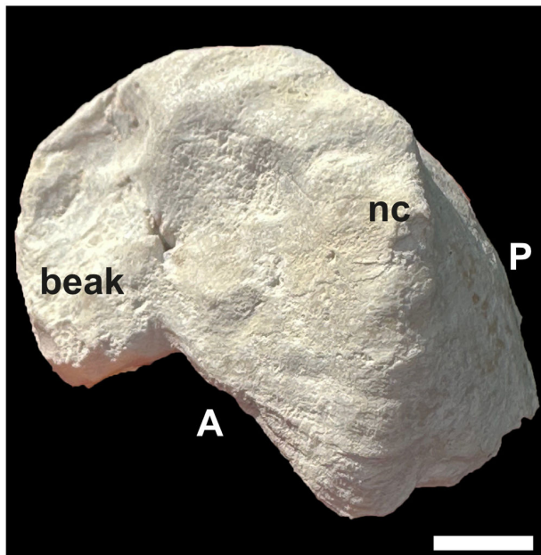
Figure 8: Requieria gryphoides MATHERON from Aiguèze. View of a LV showing the ventral nodulous carina (nc) and short beak (JPMA 18136a). Scale bar 10 mm.
