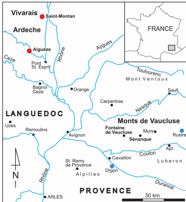
Figure 1: Geographical location of Barremian-lower Aptian Urgonian sites of Provence and Languedoc. The key localities for rudist faunas are in red. Reference localities used for comparisons are in blue.
