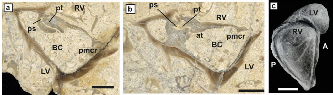
Figure 6: Matheronia aff. aptiensis MATHERON. a-b ) Oblique dorso-ventral pair sections of a bivalve specimen showing the internal characters (SU.PAL.2022.1.15.14.1) from Saint-Montan. c ) Matheronia aptiensis from Orgon (reproduced from Pl. III, fig. 6 in PAQUIER, 1903). Scale bar 10 mm.
