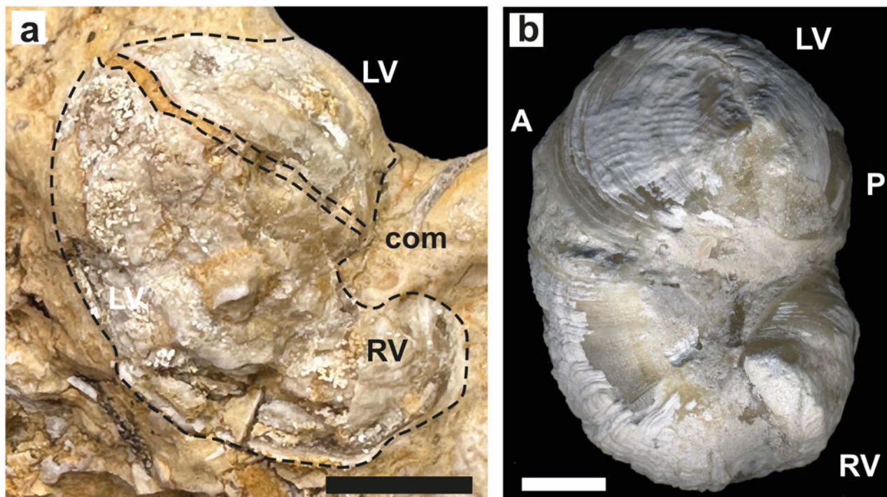
Figure 10: Monopleura varians MATHERON. a) Posterior view of a bivalve specimen from Aiguèze (JPMA 18107). b) Specimen from Orgon (reproduced from MASSE et al. , 2020: Fig. 7, H). Scale bar 10 mm.
