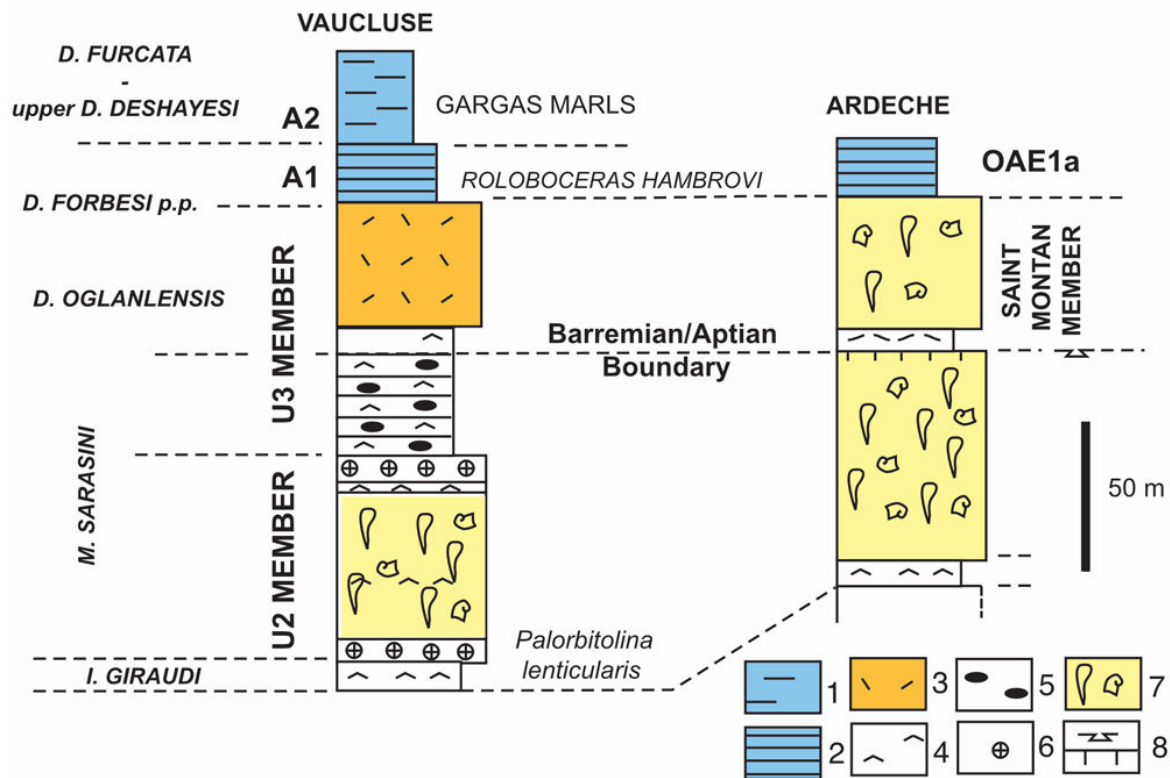
▼ Figure 4: Stratigraphic correlations between the upper Barremian-lower Aptian Urgonian successions of the Monts de Vaucluse and Ardèche (modified from MASSE et al. , 2020: Fig. 10).
