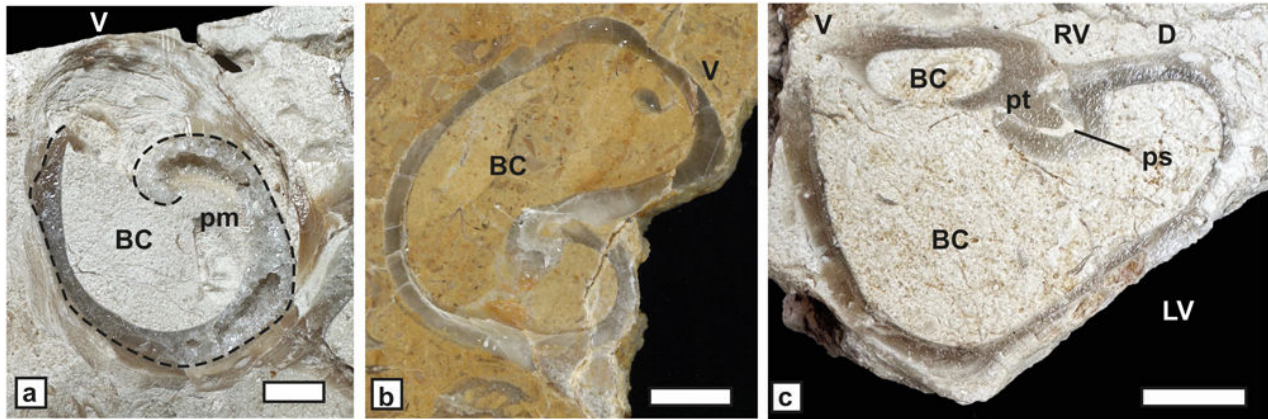
Figure 7: Requieria ammonia (Goldfuss) from Aiguèze. a) External view of a RV showing the spirograte underlined track of the posterior myophore (JPMA 18082-1A). b) Dorso-ventral oblique section of a LV showing the coiling habit and thickened, convex calcitic outer shell (SU.PAL.2022.1.15.12.1). c) Dorso-ventral section of a bivalve specimen showing the RV myophore and the spoon-like shape of the posterior socket of LV and salient tooth of RV (JPMA 18090). Scale bar 10 mm.
