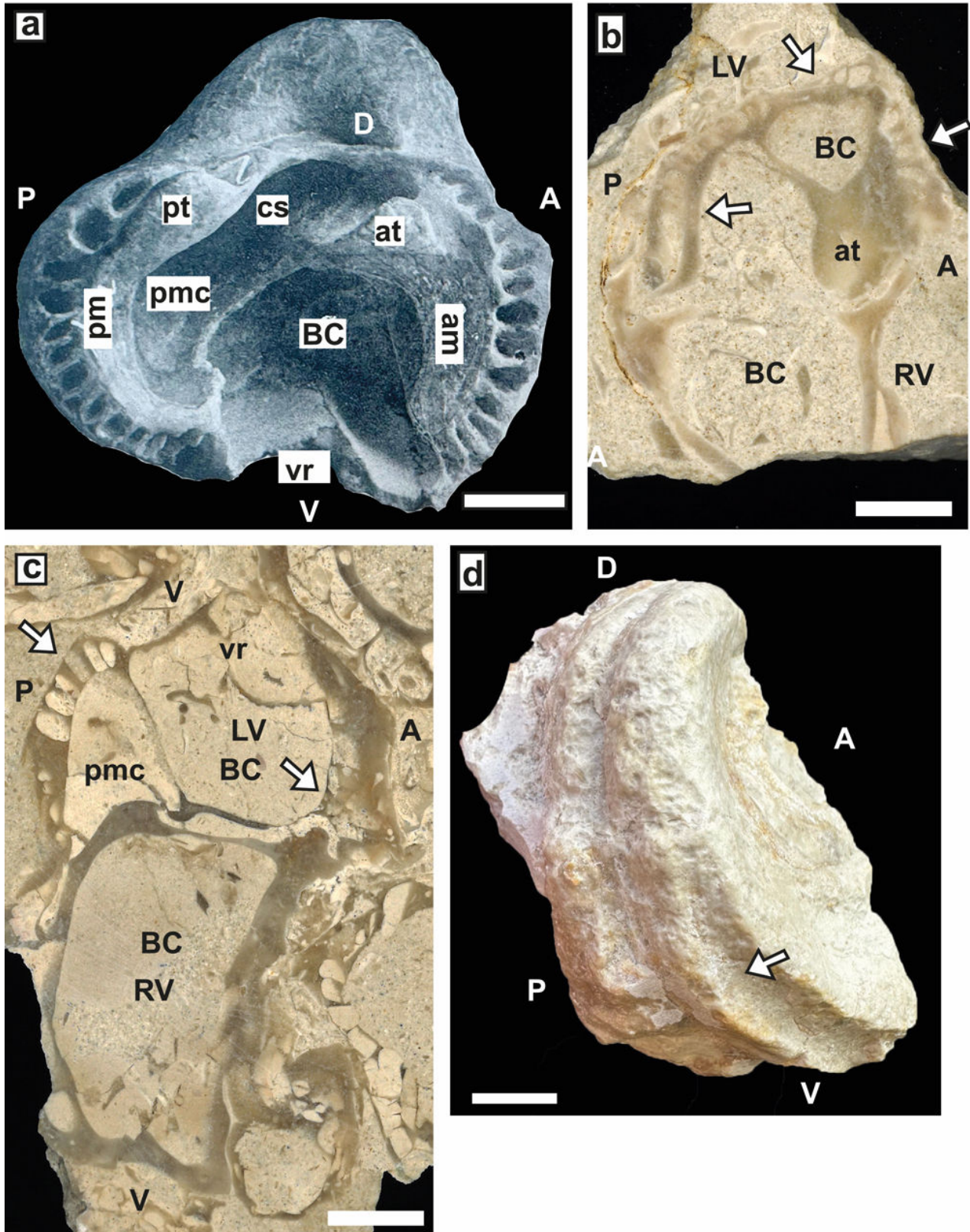
Figure 22: Praeacprina cf. varians PAQUIER. a) LV of Praeacprina varians from Saint-Montan, reproduced from PAQUIER, 1905 (Pl. VIII, fig. 7). b) Longitudinal section of a bivalve specimen showing the coiling of the LV from Cité du barrage (SU.PAL.2022.1.15.5.3). c) Longitudinal oblique sections of conjoined valves from Cité du barrage (SU.PAL.2022.1.15.5.4). d) LV internal mold showing the coiling and the tracks of the internal cavities (arrow), from Aiguèze (JPMA 18066-1). Scale bar 10 mm.
