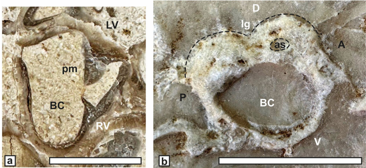
Figure 13: Debrunia occitanica MASSE & FENERCI-MASSE. a) Longitudinal section of a bivalve specimen showing the posterior myophoral organization, from Aiguèze (JPMA 18177-2). b) Transverse section of a RV showing the bilobate dorsal side, from Saint-Montan (JPMA 18062a). Scale bar 10 mm.
