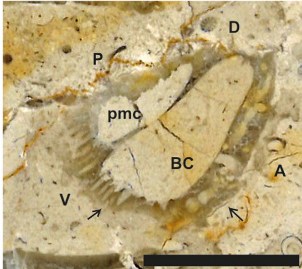
Figure 27: Caprina douvillei PAQUIER. Section of a LV showing the body and posterior myophoral cavity, and the antero-ventral canaliculation (arrows). Trescouvieux. Scale bar 10 mm.
