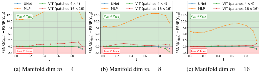
(a) Manifold dim m = 4
