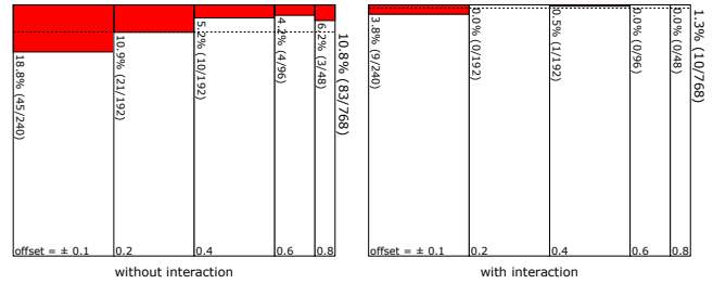
Figure 7: Rates and distributions of order errors, left: without interaction; right: with interaction. The rectangles represent the offsets between the targets. The widths of the rectangles are proportional to the number of tasks. Errors are represented by the red rectangles; the dotted line indicates the mean error rate.
