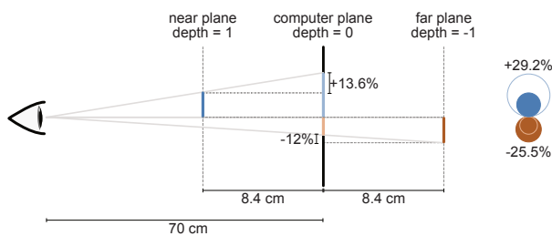
Figure 10: Size variation between projections with and without perspective. The nearest and farthest targets are positioned at \pm 8.4 cm from the central computer plane. The computer is positioned at 70 cm from the user's eyes. Under these conditions, the nearest target exhibits a 29.2% increase in size when using perspective (13.6% for its radius), and the farthest target exhibits a 25.5% decrease in size (12% for its radius).
