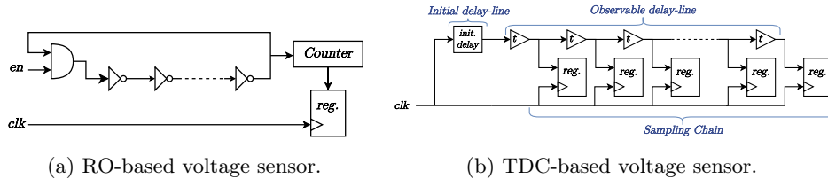
Fig. 1: Sensor types used in voltage drop detection.
