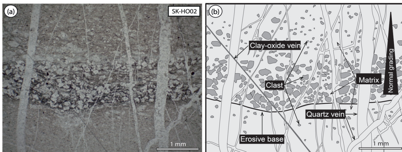
Figure 5. Illustration of clast relicts, matrix and cross-cutting veins in the black-and-white SK-HO02 chert sample from the Hooggenoeg 3 section. Note the presence of an erosive base and the normal grading of clasts upwards in the sedimentary layer. (a) represents a microphotograph and (b) is an interpretation sketch drawing interpreting this microphotograph and illustrating the different quartz types and veins that are present in the rock.
