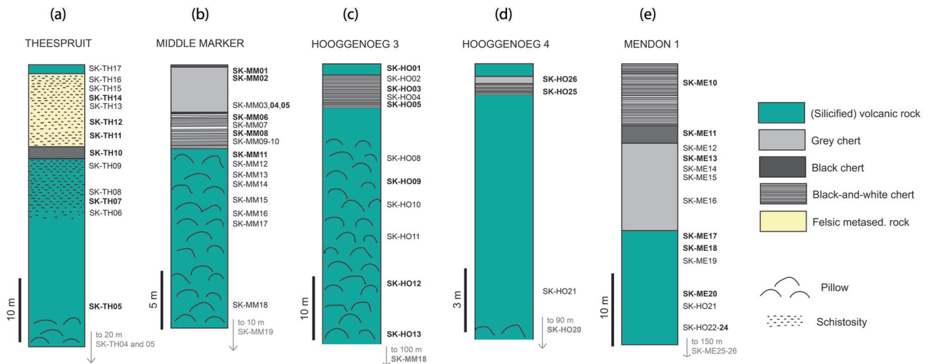
Figure 2. Detailed lithostratigraphic logs of the studied localities with the location of collected samples: (a) Theespruit section, (b) Middle Marker section, (c) Hooggenoeg 3 section, (d) Hooggenoeg 4 section, (e) Mendon 1 section. The location of each stratigraphic section on the geological map and stratigraphic succession of the Barberton Greenstone Belt is shown in Figure 1. In bold are samples that were selected for major and trace element, isotopic and thermometric analyses.
