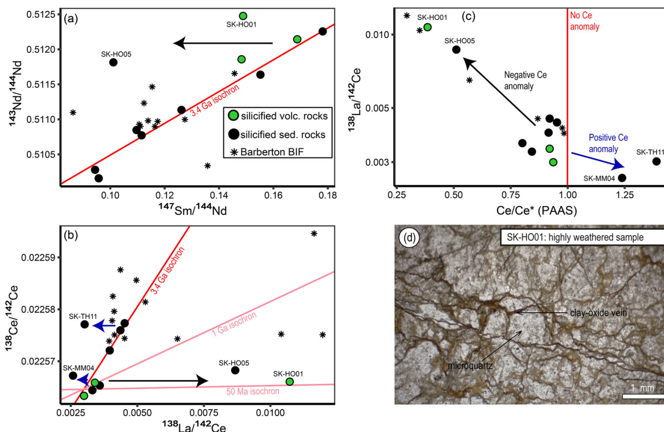
Figure 10. Results for (a) La-Ce and (b) Sm-Nd isotopic systematics measured in selected silicified volcanic and sedimentary rock samples represented in isochron diagrams. (c) ^{138}\text{La}/^{142}\text{Ce} versus \text{Ce}/\text{Ce}^*_{\text{PAAS}} . In (a) and (b) the red oblique lines represent a theoretical isochron of \sim 3.4 Ga-old material starting from a chondritic isotopic composition, and in (c) shows the position of samples that are free of Ce anomalies. Isochrons of different ages are represented in (b). They are anchored near the current La-Ce isotopic composition of mafic samples that are almost free of Ce anomalies. The alignment of most samples along theoretical isochrons suggests that the parent/daughter ratios of the studied rocks have not been significantly modified by post-Paleoproterozoic processes. Two samples fall off the regression lines for both isotopic systematics, SK-HO05 (chert) and SK-HO01 (volcanic rock sample). These two samples characterised by negative Ce anomalies deviate to the right-hand side of the ^{138}\text{La}/^{142}\text{Ce} - ^{138}\text{Ce}/^{142}\text{Ce} regression ( ^{138}\text{La}/^{142}\text{Ce} increase). Additionally, samples SK-TH11 and SK-MM04 showing positive Ce anomalies deviate to the left-hand side of the ^{138}\text{La}/^{142}\text{Ce} - ^{138}\text{Ce}/^{142}\text{Ce} regression ( ^{138}\text{La}/^{142}\text{Ce} decrease). These results prove that the La/Ce fractionation reflected by Ce anomalies is not pristine but reflects post-depositional processes. Panel (d) shows a microphotograph of the highly altered SK-HO01 silicified volcanic rock sample, depicting late-stage veins of clay and oxides. Note that error bars are smaller than the size of symbols. For comparison, isotopic data of Barberton BIF samples from the Fig Tree and Moodies units that were previously published by Hayashi et al. (2004) and Bonnand et al. (2019) are also reported.
