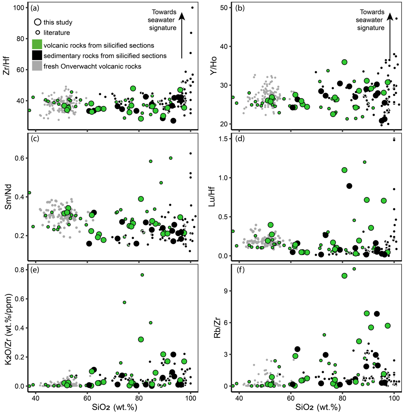
Figure 8. Evolution of selected elemental ratios with increasing \text{SiO}_2 concentration. (a) and (b): \text{SiO}_2 versus Zr/Hf and Y/Ho ratios for which silicified volcanic rocks generally remain within the range of fresh volcanic rocks for these ratios. (c): \text{SiO}_2 versus Sm/Nd showing that this ratio decreased slightly during silicification. (d): \text{SiO}_2 versus Lu/Hf ratio showing significantly variable Lu/Hf ratios in silicified volcanic (and sedimentary) rocks compared to fresh volcanic rocks. (e) and (f): \text{SiO}_2 versus \text{K}_2\text{O}/\text{Zr} and Rb/Zr ratio. We note higher \text{K}_2\text{O}/\text{Zr} and Rb/Zr ratios in silicified rocks compared to fresh volcanic rocks. References for the comparison data compiled from previous studies are given in Figure 4 caption.
