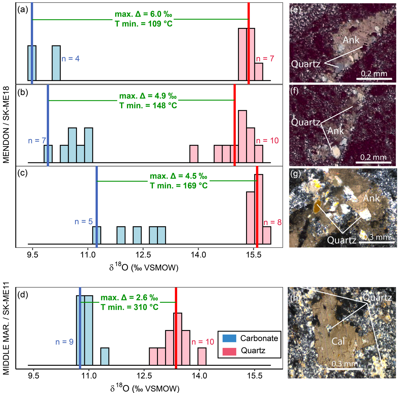
Figure 7. Histograms showing the distribution of \delta^{18}\text{O} values and equilibrium temperatures obtained from analysed quartz (reddish) and carbonate (bluish) assemblages. (a), (b) and (c) present results of analyses in individual assemblages of the silicified volcanic rock sample SK-ME18 of the Mendon section. (d) presents results obtained from the single assemblage of the silicified volcanic rock sample SK-MM11 that we analysed. Vertical lines show mean quartz \delta^{18}\text{O} values (red) and minimum carbonate \delta^{18}\text{O} values (blue). The reported minimum temperatures were calculated using the following equation: maximum \Delta = 0.87 (\pm 0.06) \times 10^6 / T^2 (Clayton et al., 1972; Sharp and Kirschner, 1994), with maximum \Delta = \text{mean } \delta^{18}\text{O}_{\text{quartz}} - \text{minimum } \delta^{18}\text{O}_{\text{carbonate}} . (e), (f), (g) and (h) show the petrography of the quartz-carbonate assemblages whose O isotope compositions are respectively displayed in (a), (b), (c) and (d).
