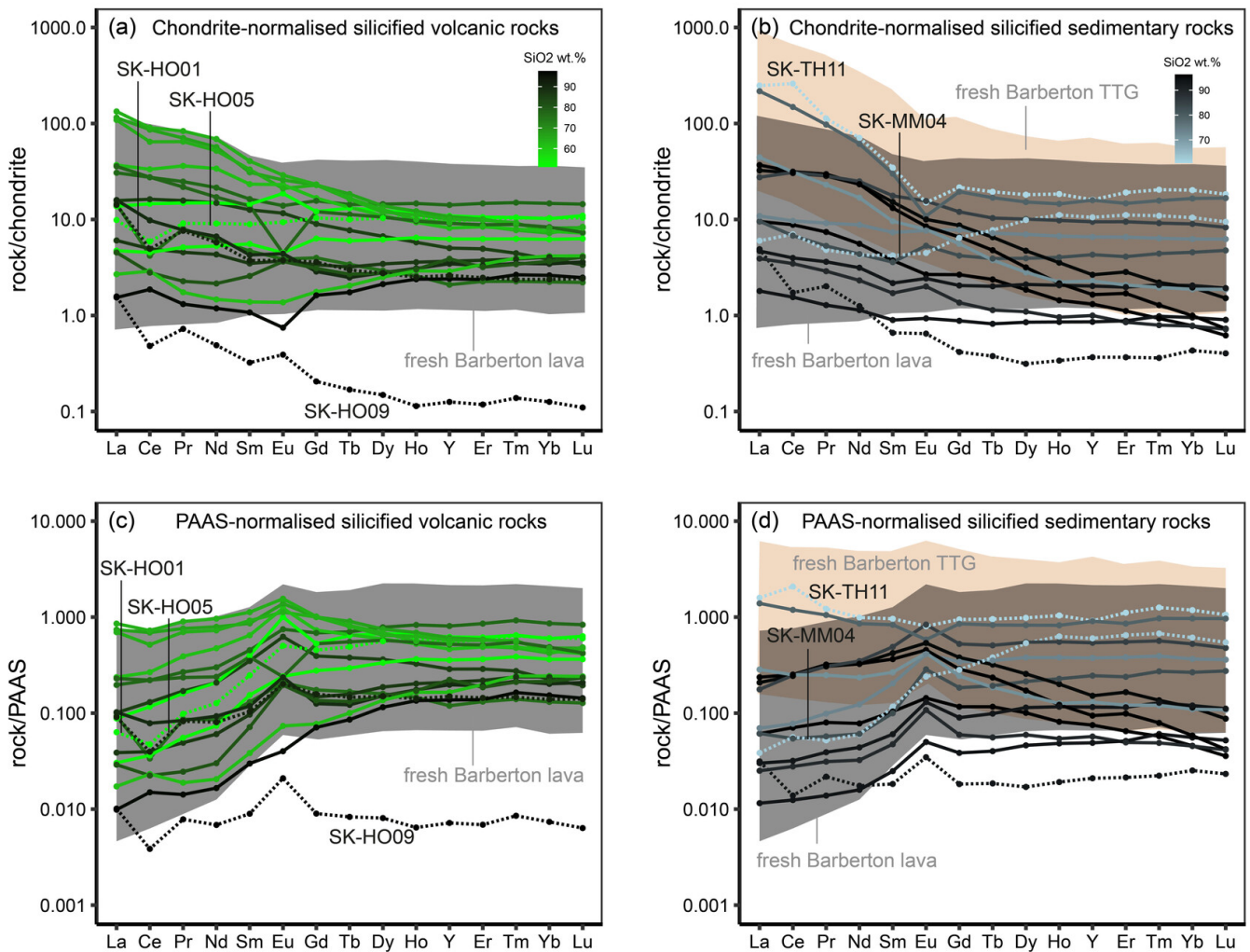
Figure 9. Chondrite (a and b) and PAAS (c and d) normalised REE patterns of the analysed silicified volcanic and sedimentary rock samples. Chondrite values are from Anders and Grevesse (1989) , and PAAS values are from Taylor and McLennan (1985) . Colour-coding based on \text{SiO}_2 concentration illustrates that the REE content of the analysed samples decreases with increasing \text{SiO}_2 concentration. For comparison, we report the field of REE patterns measured in fresh Onverwacht volcanic rocks ( Chavagnac, 2004 ; Furnes et al., 2012 ; Lahaye et al., 1995 ; Parman et al., 2001 ; Puchtel et al., 2013 ; Schneider et al., 2019 ) and in Barberton granitoids ( Moyen et al., 2019 ). Samples highlighted with dotted lines, including SK-HO01, SK-HO05, SK-HO09, SK-TH11, SK-MM04, exhibit pronounced Ce anomalies discussed in the full text.
