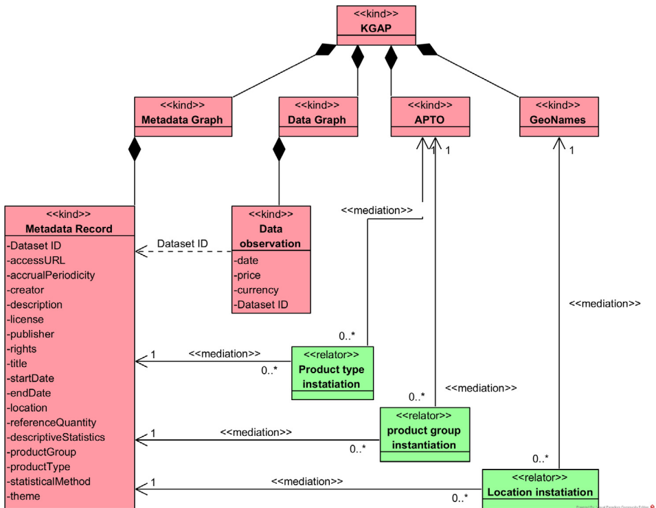
Fig. 1. KGAP OntoUML Conceptual Model.
