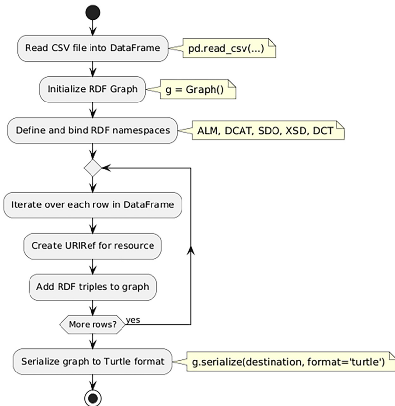
Fig. 2. Metadata Converter Pipeline.
