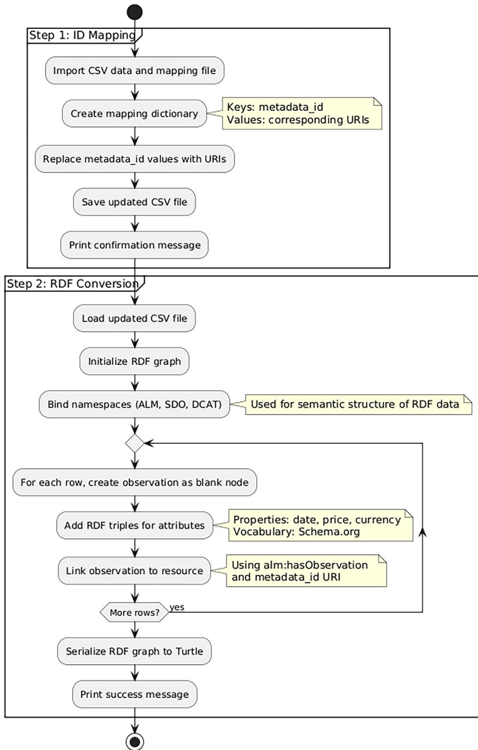
Fig. 4. Data Converter Pipeline.
