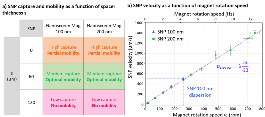
Fig. 5 SNP mobility and velocity range. (a) Table summarizing SNP capture and mobility for different spacer thicknesses s = \{0 \mu\text{m}, 60 \mu\text{m}, 120 \mu\text{m}\} . (b) Experimental SNP velocity ( \mu\text{m s}^{-1} ) on 60 \mu\text{m} -thick spacer as a function of external magnet rotation speed \omega (rpm). Blue triangles and green circles represent 100 nm and 200 nm SNPs respectively. Dashed purple line represents theoretical SNP drive velocity as a function of magnet rotation speed. Dashed horizontal and vertical blue lines points critical speed and corresponding magnet rotation speed for 100 nm SNPs. Vertical error bars represent standard deviation of measurements extracted from a dataset of n = 3 independent experiments. Horizontal error bars correspond to the error in the experimental measurement of the external magnetic field rotation rate using a Hall probe. The twin top x axis indicates the magnet rotation rate in Hz.
