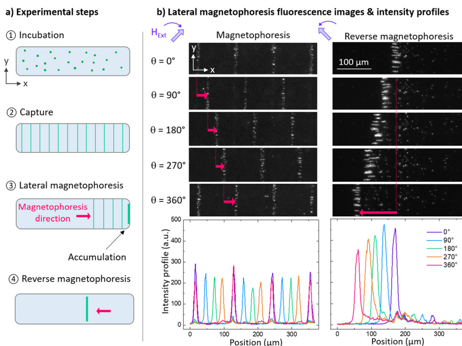
Fig. 4 SNP 1D line accumulation. (a) Schematic description of experimental steps. Step 1 (incubation): SNPs are injected into the micro-magnetofluidic chip outside the magnetophoresis platform. Thanks to the spacer, SNPs are not captured on the substrate surface, allowing them to interact with molecules of interest in the sample. Step 2 (capture): Introduction of the chip in the external magnetic field induces SNP magnetization and their subsequent capture on the magnetic line pattern. Step 3 (accumulation): Lateral magnetophoresis is activated in order to move the SNP lines and accumulate them against the right side of the fluidic chamber. Step 4 (repositioning): Magnetophoresis is reversed in order to displace the concentrated SNP line back towards the center of the chip. (b) Positions at different external magnetic field angles \theta of several SNP lines when rotating the field clockwise (left) and of a single 1D accumulated line (right) when rotating counterclockwise. Fluorescence images and corresponding fluorescence intensity profiles are presented. Related S1 and S2 movies are provided in SI.
