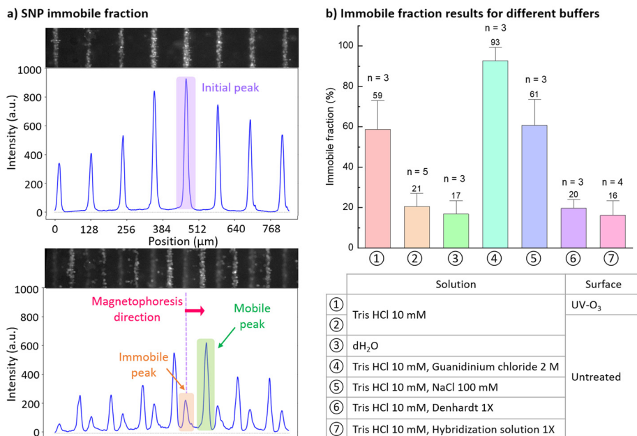
Fig. 6 Analysis of SNP immobile fraction during lateral magnetophoresis. (a) Experimental approach to determine immobile fraction. Fluorescence intensity values in acquired image are vertically integrated resulting in peaks corresponding to SNP lines captured on the substrate. Initial peak area is extracted from one frame acquired after required SNP capture time and before implementing magnetophoresis. Immobile peak area is extracted from one frame acquired after starting magnetophoresis, where SNP transport distance is inferior to the period \lambda . Immobile fraction is calculated as the average ratio between immobile and initial peaks areas. In this example, extracted immobile fraction is 26.7%. (b) Bar plot represents SNP immobile fraction in various buffer and surface conditions.
