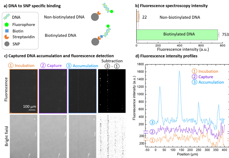
Fig. 7 SNP accumulation for DNA detection. (a) Illustration of DNA to SNP specific binding via streptavidin to biotin affinity. (b) Specificity of the interaction between biotinylated fluorescent DNA and streptavidin-coated SNPs. Biotinylated or non-biotinylated fluorescent DNA was incubated with streptavidin-coated Estapor SNPs. Fluorescence intensity was measured on SNPs resuspended in Tris HCl 10 mM after incubation and subsequent washing. (c) Fluorescence and bright field images acquired during each experimental step. (d) Fluorescence intensity vertical profiles extracted from fluorescence images, after background subtraction.
