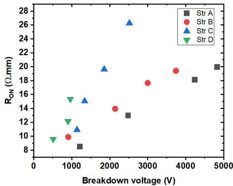
FIG. 3. Typical R_{ON} values as a function of the breakdown voltage for all GD
