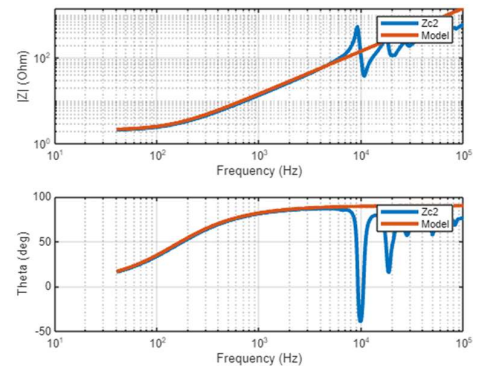
Fig.13.4. Simulation of ZC2
