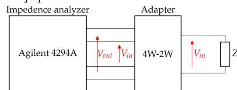
Fig.1. Impedance analysis circuit diagram.
