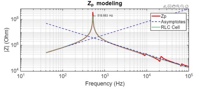
Fig.7. Z_p calculation and equivalent RLC cell representation
