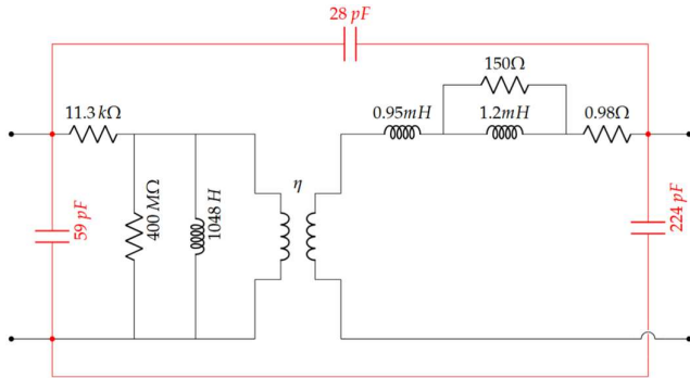
Fig.12. Simplified validation circuit implemented
