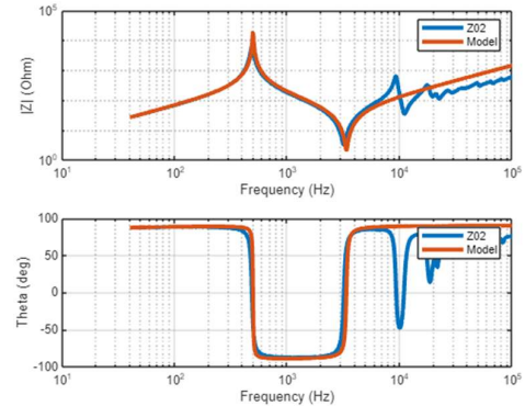
Fig.13.3. Simulation of Z02
