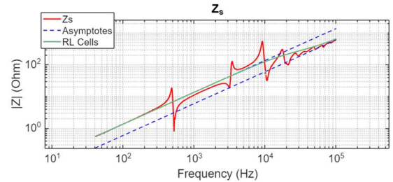
Fig.9. Z_s calculation and equivalent RL cell representation
