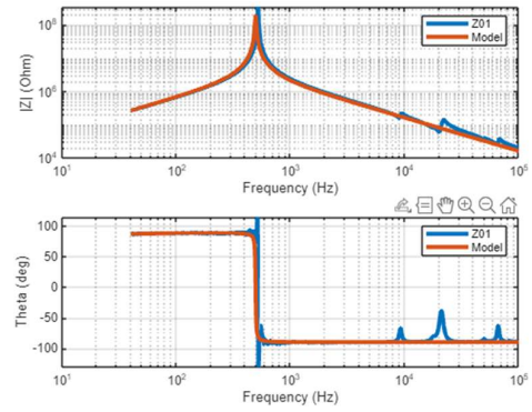
Fig.13.1. Simulation of Z01
