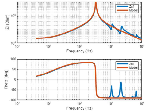
Fig.13.2. Simulation of ZC1
