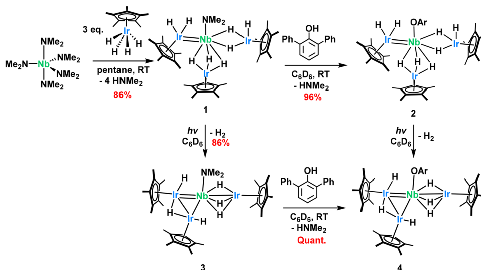
Scheme 3 The synthesis of the niobium iridium complexes.
