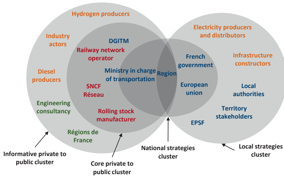
Fig. 5. Clusters representation.
