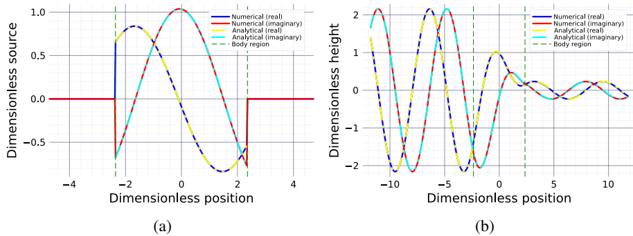
Figure 2: (a) An example of a source, \hat{Q}(x) , that results in the optimal thrust under the bounded norm constraint where \nu = 0 and l = 3\pi/2 . (b) The corresponding wave-field, \hat{h}(x) under the same conditions.
