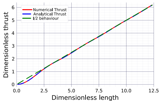
Figure 3: Plot of the time-averaged thrust \bar{F}_T vs the dimensionless length scale l resulting from the bounded norm optimisation on start-up \nu \approx 0 . It can also be seen that as l increases, the dimensional thrust tends to scale with \frac{l}{2} which is the same behaviour found in (3.9) for l \gg 1
