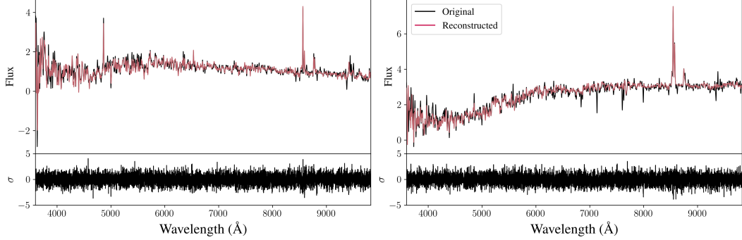
Figure 10: Spectrum Tokenizer Performance: Reconstruction quality of the spectrum tokenizer on two representative DESI EDR spectra. Top panels show the normalized flux as a function of wavelength, with original input (black) and reconstructed output (red) overlaid. Bottom panels show the residuals in units of the input uncertainty ( \sigma ).
