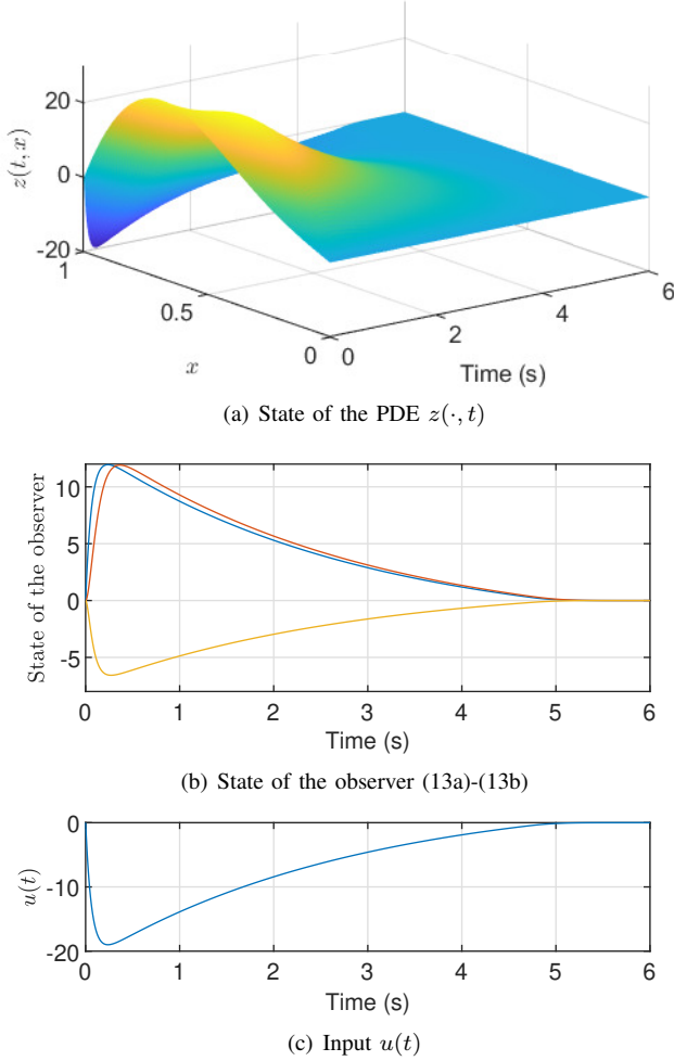
Fig. 1. Time-domain behavior of the closed-loop system from the initial condition z_0(x) = 10(1 + 5x^2) \sin(\pi x)
