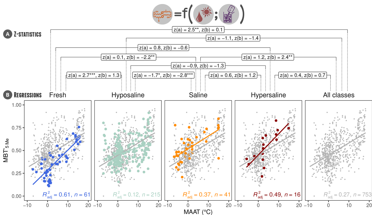
Figure 11. Effect of salinity (i.e., the TDS of each surface sample) on the linear relationship between temperature (here MAAT) and the MBT'_{5Me} . Panel (A) shows the results of the z-statistic tests assessing significant differences in slopes and intercepts between salinity classes. Panel (B) presents linear regressions for fresh, hyposaline, saline, and hypersaline classes, based on the full ACADB. For each salinity group, temperature calibrations of the form MAAT = a \times MBT'_{5Me} + b are proposed (B). The z-statistic method (Clogg et al., 1995) evaluates the significance of slope ( a ) and intercept ( b ) differences across two classes (grey lines link the two classes with their z-statistics on panel A). The p values of the z-statistic are displayed with *** for p \leq 0.01 , ** for p \leq 0.05 , and * for p \leq 0.1 .
