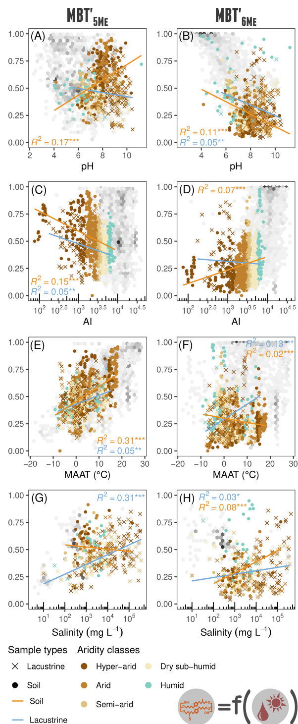
Figure 6. MBT'_{5Me} and MBT'_{6Me} relationships with pH (A, B), Aridity Index (C, D), MAAT (E, F), and salinity (G, H). The colour refers to the aridity classes for the samples. Two groups per sample type (i.e., lacustrine and soil) are used to infer linear relationships. The grey hexagonal bins show the sample density from the WDB. R^2 values are shown only for statistically significant regressions ( p < 0.05 ), while p values below 0.001, 0.01, and 0.05 are indicated with ***, **, and *, respectively.
