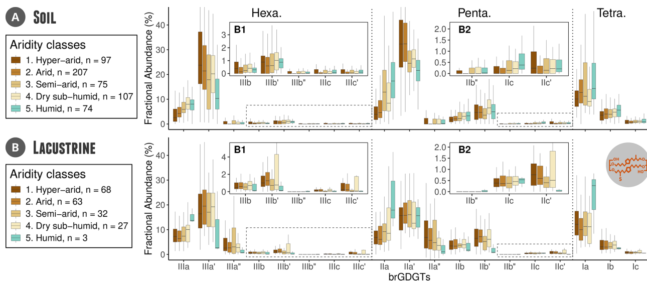
Figure 3. Distribution of individual brGDGTs grouped by aridity index, following the five aridity classes (Middleton and Thomas, 1997) in the ACADB for soil (A) and lacustrine samples (B). The brGDGT fractional abundances (FA) are displayed with ' for the 6-methyl and '' for the 7-methyl isomers. The hinges of the boxplots show the 25 % (Q1) and 75 % (Q3) quantiles, the middle horizontal line indicates the median, and the whiskers extend to the most extreme data points that lie within 1.5 \times the inter-quartile range (i.e., Q3 - Q1 ). Points beyond the whiskers are considered outliers and are not shown here. The compounds of lowest abundances (mean value below 5 %) are zoomed on panels (A1), (A2), (B1) and (B2).
