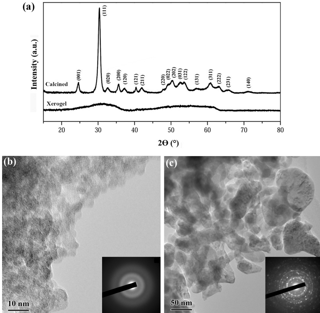
Fig. 1. XRD pattern of the xerogel and calcined powder (a), TEM micrograph and SAD pattern of the xerogel (b), and TEM micrograph and SAD pattern of the calcined powder (c).
