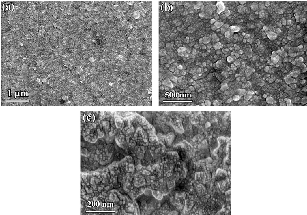
Fig. 3. SEM micrograph of the film which signifies the film quality at a low magnification (a) and SEM micrograph at higher magnifications obtained at a working voltage of 20 kV (b) and 2 kV (c).
