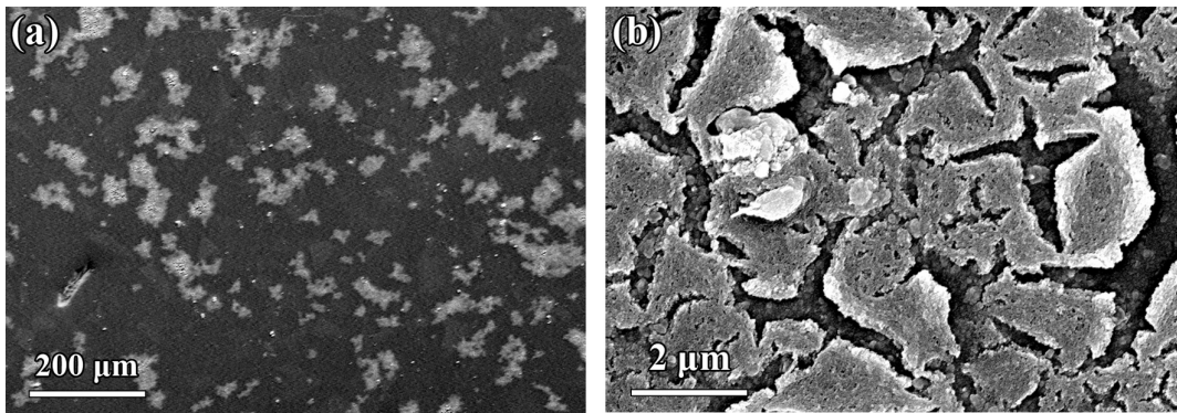
Fig. 2. SEM micrograph of the film deposited in the absence of CMC, in a low magnification (a) and in a higher magnification (b).
