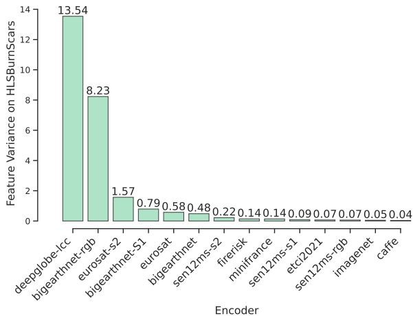
Figure 3. Variance of the feature maps computed by different encoders on the HLS Burn Scars training set. The variance changes a lot between encoders, which could create problems when training an ensemble.
