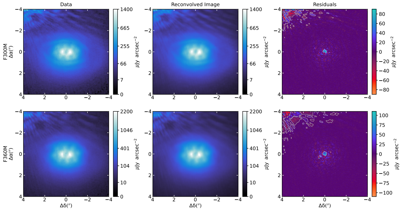
Figure 14. The same as in Figure 6, but for reconvolution of the deconvolved images following the procedure outlined in Appendix B. Gray contours in the right column indicate \pm 3\sigma thresholds for the residuals. To approximate the noise level for this purpose, we adopt the propagated pixel-wise uncertainties from the ERR FITS extensions. As these estimates neglect residual speckle noise, they should be assumed to underestimate the noise where speckle residuals are nonnegligible (at very small separations and near the M dwarfs). The residual maps used for the contours were convolved with an FWHM-diameter tophat filter, which serves to mitigate the appearance of the single-pixel deviations expected from Gaussian noise but does not qualitatively alter the result.
