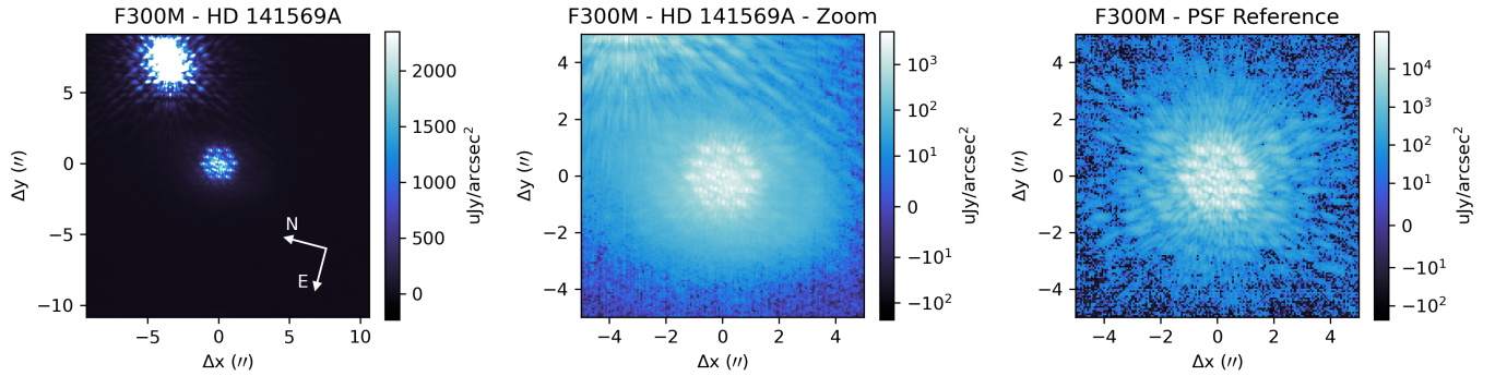
Figure 1. Left panel: a view of the entire coronagraphic F300M field of the HD 141569 system. The two unocculted M-star companions are located to the upper left. The color map has been chosen to highlight the coronagraphic PSF and as a result the M-star PSF cores visually appear saturated. In reality, the detector has not been saturated by the M-stars. Center panel: a zoom in on the central regions of HD 141569A, shown with a log image normalization. Right panel: a zoom in on the central regions of the PSF reference star.
