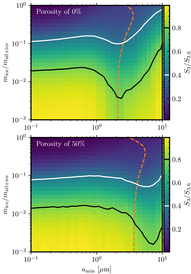
Figure 10. Expected surface brightness ratio between F300M and F360M as a function of the minimum grain size and the water ice fraction in grains (by mass). The top panel presents a case of compact grains (0% porosity), while the bottom panel presents a porous case (50% porosity). The white and black contours represent a brightness ratio of 0.4 and 0.8 as found at 100 and 400 au, respectively. The orange dashed line represents the expected minimum grain size as a function of the ice fraction.
