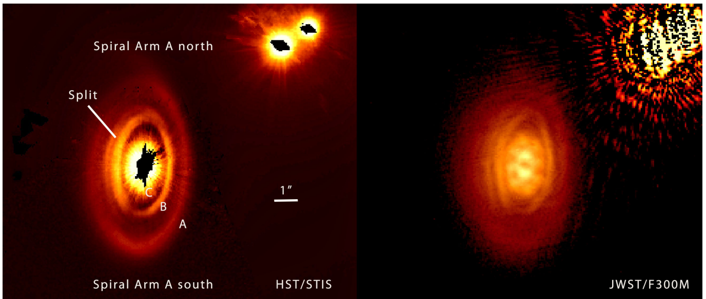
Figure 4. Comparison of disk structures between archival HST/STIS optical coronagraphic data (left panel) and the JWST/NIRCAM F300M observations (right panel). A key difference in the morphologies is that the JWST data do not show a well-defined deep gap between the A and B ring components. North is up, and east is left.
