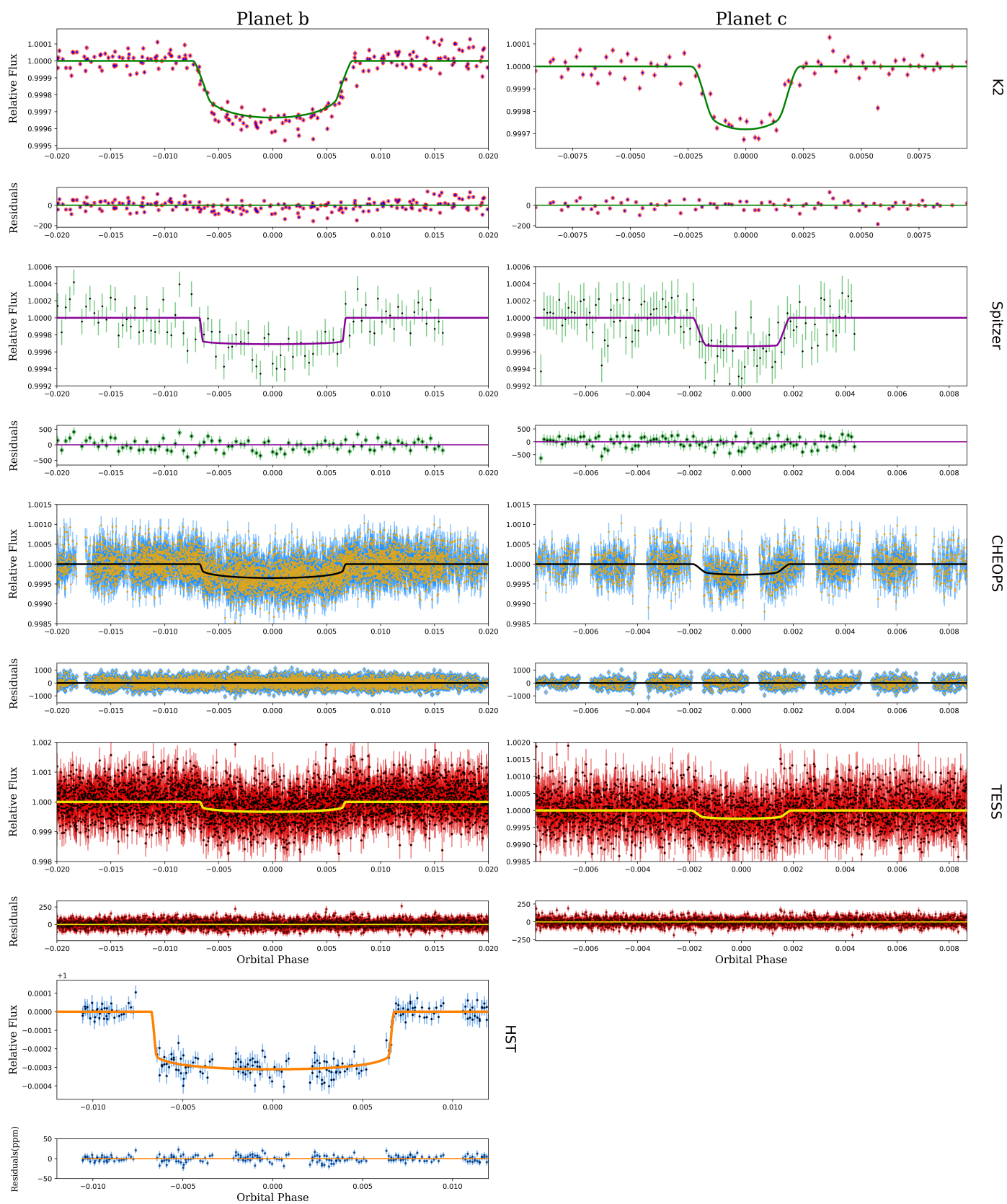
Fig. A.1: Phase-folded light curves of HIP 41378 b & c, combining observations from K2, Spitzer, HST, CHEOPS, and TESS. The oversampled best-fit transit models are overlaid on the light curves.
