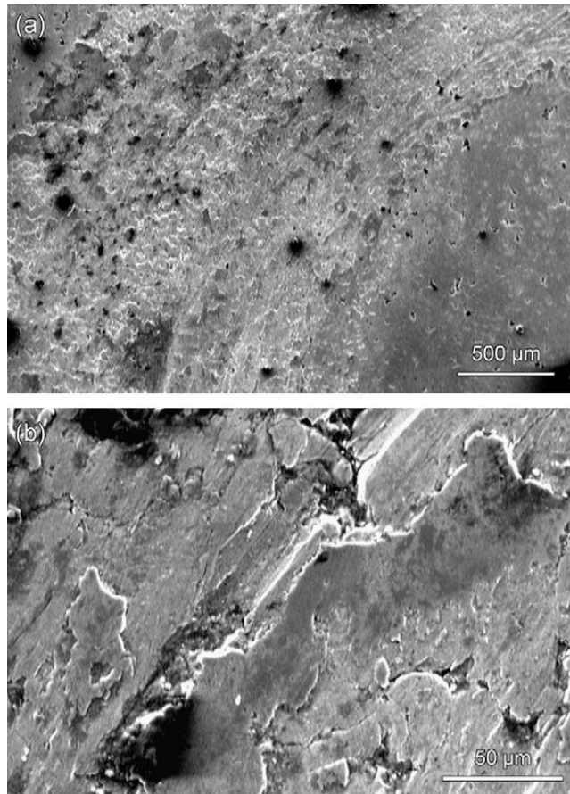
Fig. 5. SEM picture of the worn surface of the nickel-free stainless steel sample after 800 m sliding distance in two magnifications.
