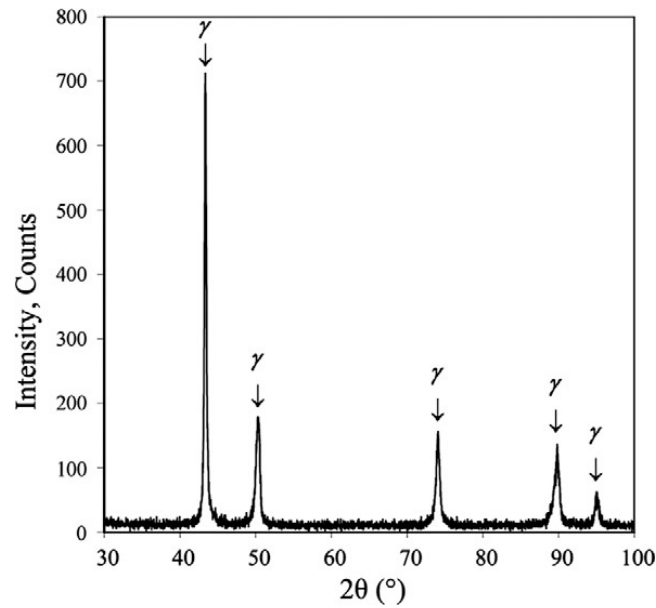
Fig. 2. XRD trace of the sample sintered at 1100 °C for 20 h and water-quenched.
