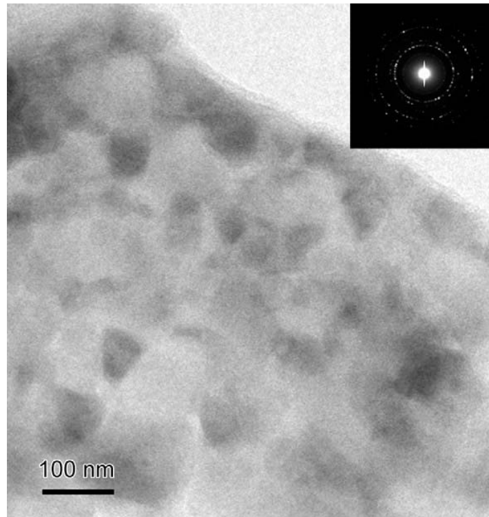
Fig. 3. TEM image and corresponding SAD pattern of the sintered material.
