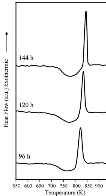
Fig. 3. DSC profiles of the amorphous samples.
