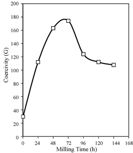
Fig. 8. The variation of coercivity with milling time.
