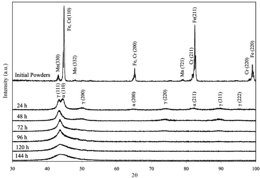
Fig. 1. XRD patterns of the as-milled powders.
