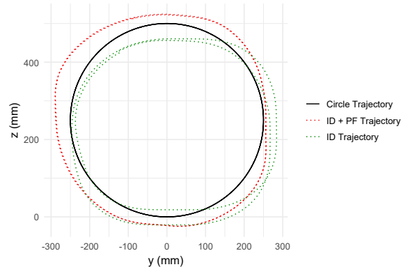
Trajectory in the plane (y,z) over two periods
