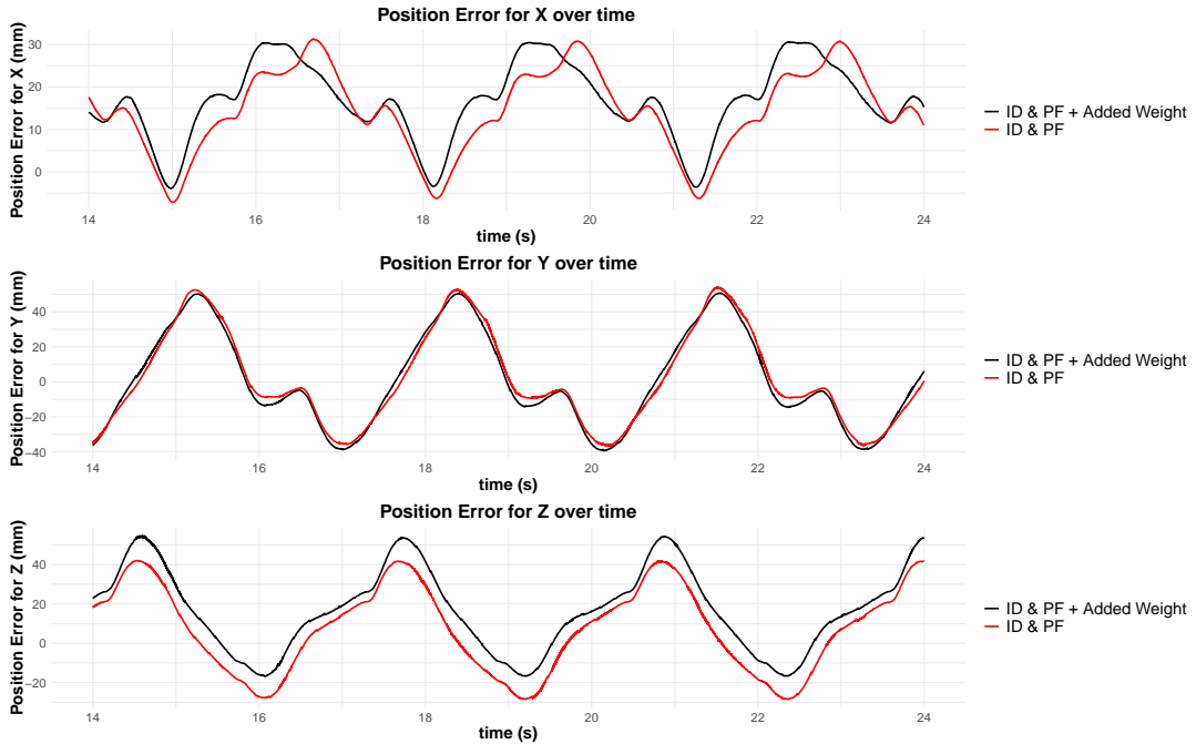
Fig. 5: Position tracking error comparing the case with and without unmodeled load, both running with ID + PF.
