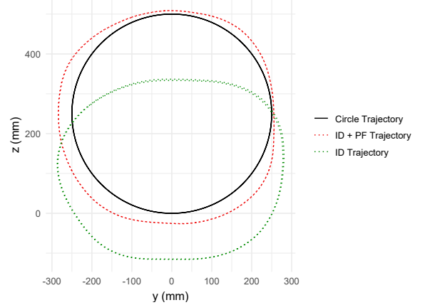
Fig. 4: End-effector trajectory in the ( y, z ) plane, under unmodeled load, over two periods with just the ID or the ID + PF in comparison to the expected circle trajectory.
