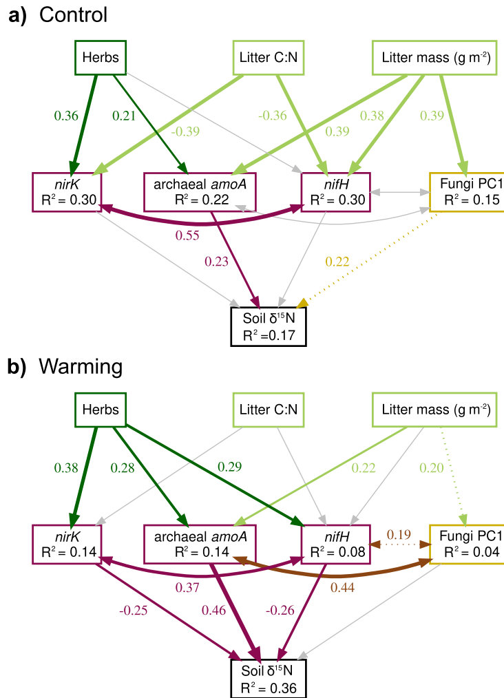
FIGURE 4 | Structural equation models showing the influence of litter properties and microbial factors on soil N isotopic signature. Multi-group structural equation models the links between herb abundance and litter properties (C:N ratio, dry weight (DW m -2 )), microbial community components (fungal community attributes PC1, and the abundance of nirK for denitrification, amoA for ammonia oxidizing archaea, and nifH for nitrogen fixation, all expressed in copies g -1 DW litter) and soil N isotopic signature (soil δ 15 N) in control (a) and warmed (b) plots. PC1 reflects increasing fungal abundance and richness and decreasing fungal evenness (Figure S4A). Correlations are depicted by double arrows, regressions by one-sided arrows, with width proportional to the indicated standardized estimate of the regression. The coefficient for the relationship is shown for significant relationships (dashed paths have p < 0.1 , solid paths p < 0.05 and grey paths p > 0.1 ). Paths were pruned when not significant in at least one treatment. Standardized coefficients of the proportion of variation explained for each non-exogenous variable are indicated in the boxes. The multi-group model was robust with \chi^2 = 23.70 , with 25 df, p = 0.65 , RMSEA = 0.000 (upper ci = 0.081, lower ci = 0.000), CFI = 1, and SRMR = 0.051.
