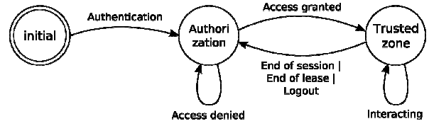
Fig. 2 Quasi-static authorization.
