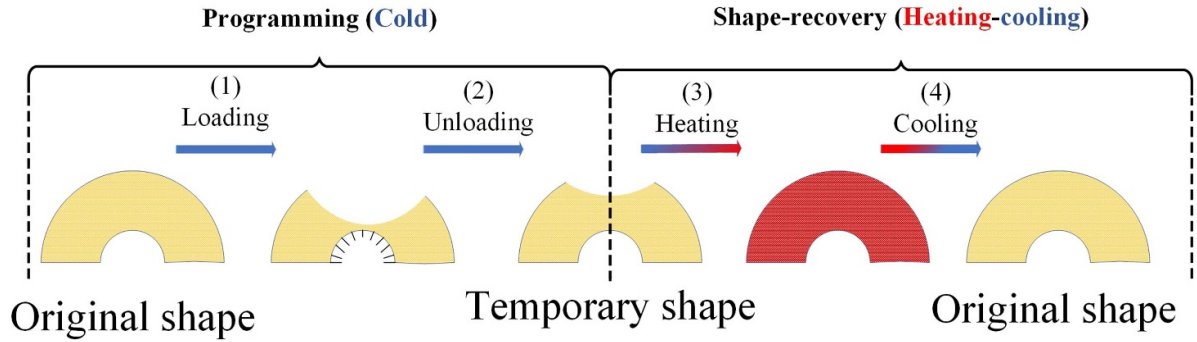
Figure 3. Description of the cold programming and shape recovery for SMP-based absorbing structures: (1) loading, (2) unloading at room temperature, (3) heating above T_g , and (4) cooling to RT.
