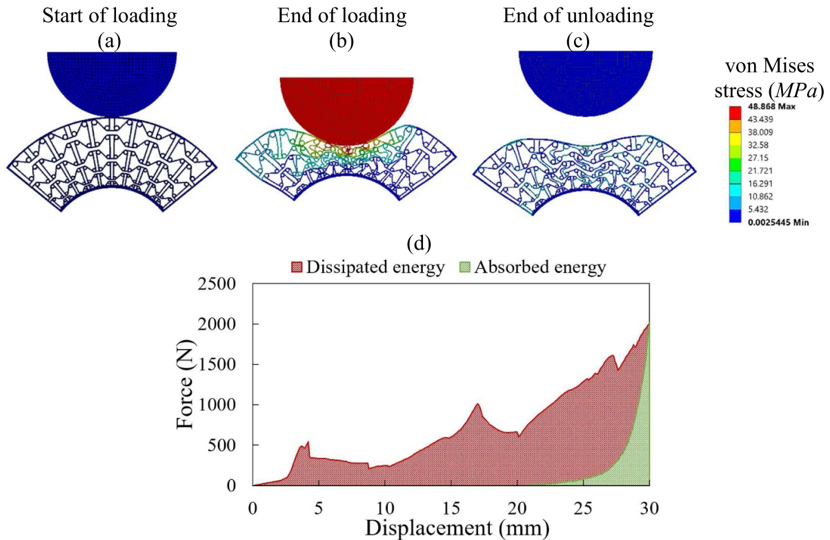
Figure 13. The counterpart of figure 11 for FG RCA I.
