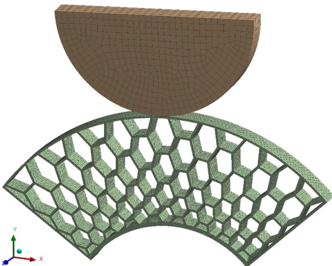
Figure 7. The lattice structure with the generated mesh.
