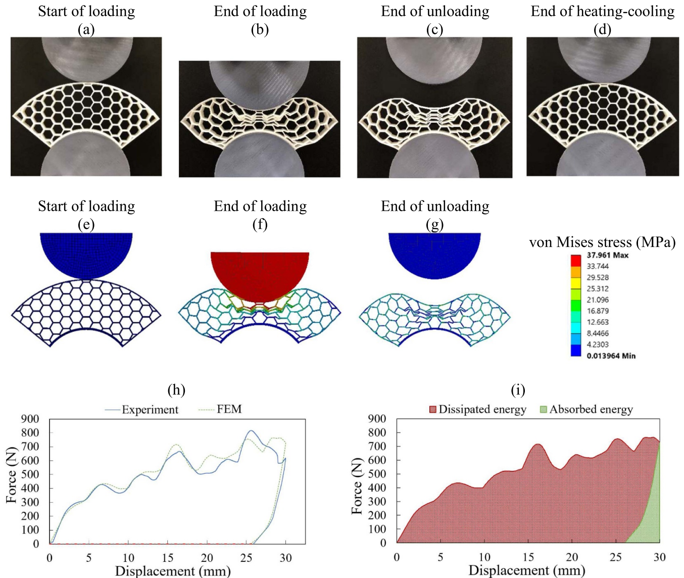
Figure 8. Uniform honeycomb: (a)–(g) experimental and computational configuration of lattice structure before loading, at the end of loading, unloading, and heating–cooling, (h) force–displacement response during loading–unloading from experiment and FEM (red dash-dotted line related to the shape-memory recovery), (i) the dissipated (red area) and absorbed energies (green area).
