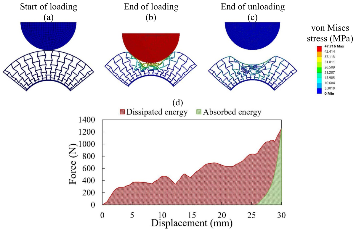
Figure 11. FG re-entrant I: (a)–(c) computational configuration of the lattice structure before loading, at the end of loading and unloading, and (d) force–displacement response during loading–unloading from FEM (dissipated and absorbed energies are denoted in red and green areas).
