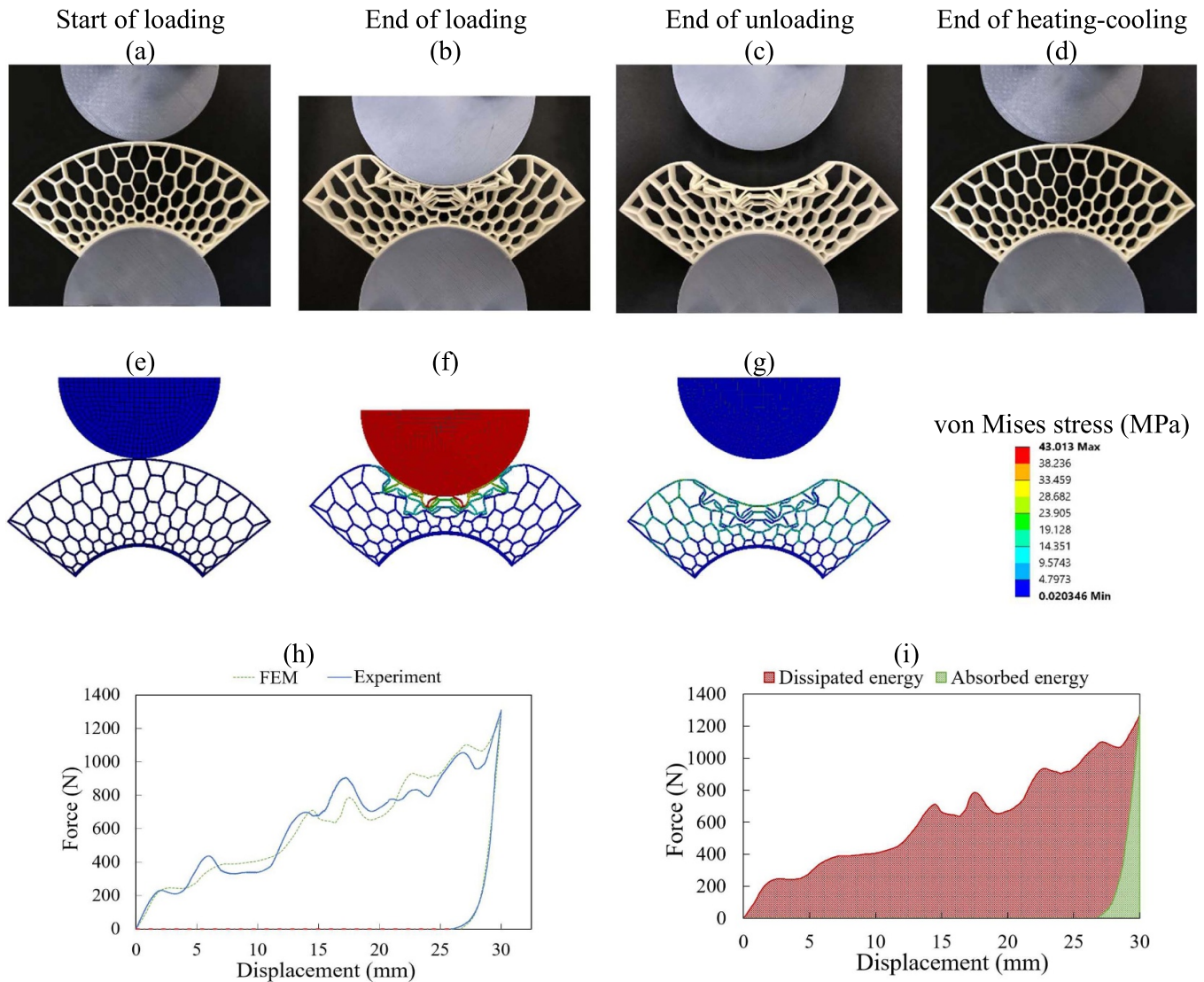
Figure 9. The counterpart of figure 8 for FG honeycomb I.
