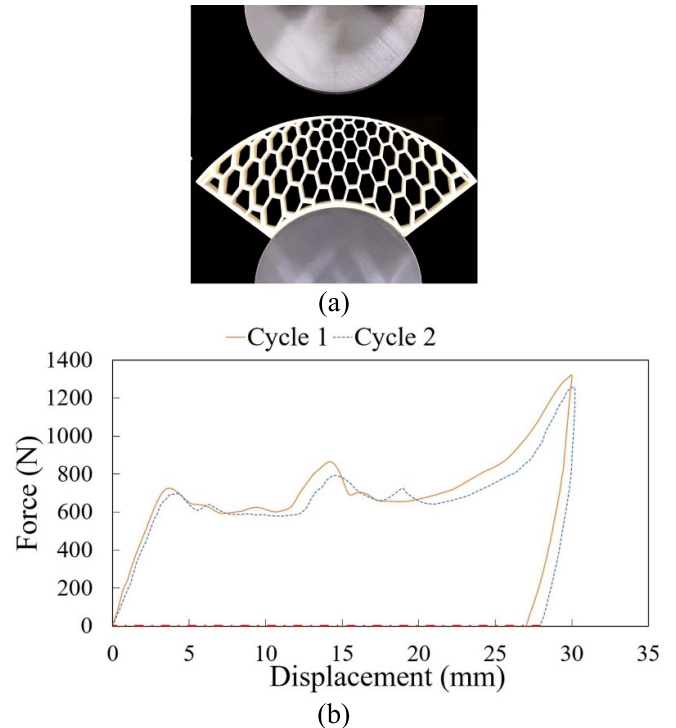
Figure 16. (a) Configuration of FG honeycomb II after heating–cooling at the end of the second loading–unloading cycle, (b) experimental force–displacement response during two cycles of loading–unloading–heating–cooling.
