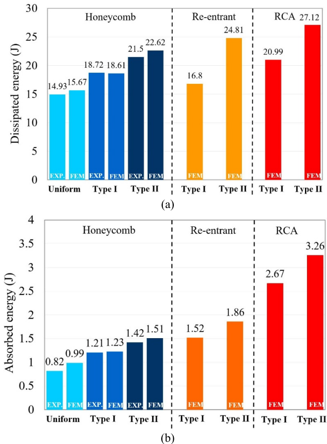
Figure 15. (a) Energy dissipation and (b) energy absorption capacity of the investigated metamaterials.
