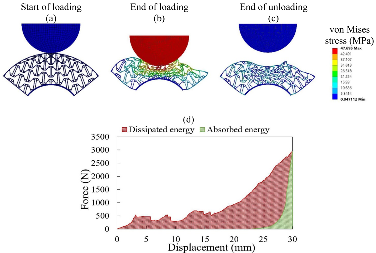
Figure 14. The counterpart of figure 11 for FG RCA II.
