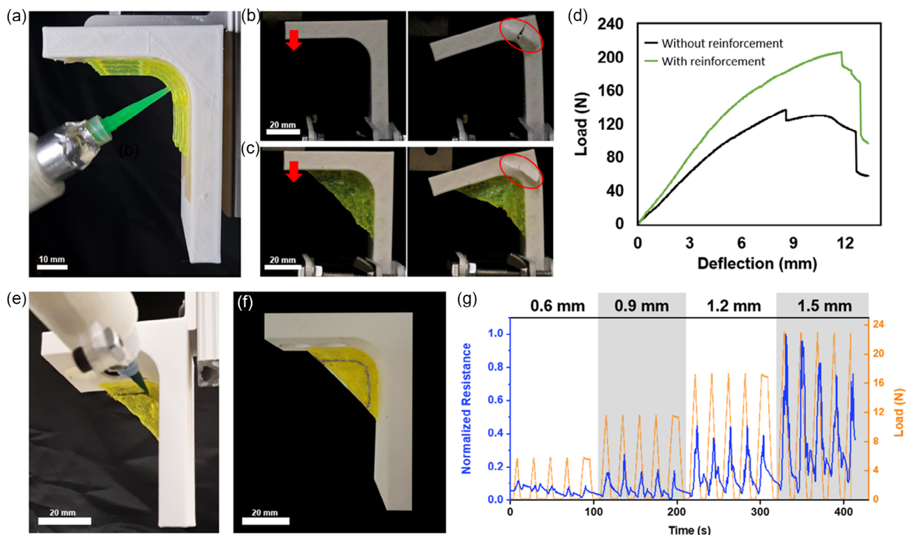
Figure 5. Multidimensional fabrication on an inverted “L”-shaped right-angle bracket. a) Fabricating a high-strength reinforcement on the bracket. b) Mechanical loading on an unreinforced bracket t = 0 (left), moment of failure (right). c) Mechanical loading on a bracket with printed reinforcement t = 0 (left), moment of failure (right). d) Graph depicting load versus deflection behavior of the reinforced and unreinforced brackets. e) Depositing a conductive path onto the surface of the printed reinforcement. f) A functional structure for sensing deflection of the bracket with respect to load. g) Normalized resistance (blue) and force (orange) responses to 0.6, 0.9, 1.2, and 1.5 mm deflections over time.
