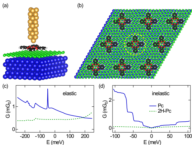
FIG. 3. (a) Side and (b) top view of the unit cell used in the simulations. (c) Elastic electron transmission function for Pc (solid line) and 2H-Pc (dashed line) as a function of energy ( E_F = 0 ). (d) Inelastic electron transmission for Pc and 2H-Pc. G_0 denotes the quantum of conductance.
