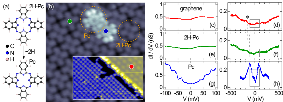
FIG. 1. (a) Ball-and-stick models of 2H-Pc and Pc. (b) STM image of molecule-covered graphene on Ir(111) (sample voltage: 0.78 V, tunneling current: 25 pA, size: 8 nm \times 8 nm). A 2H-Pc and Pc molecule are marked by dashed circles. Inset: Overview STM image with 2H-Pc-covered graphene (left) adjacent to pristine graphene (right) with the characteristic hexagonal moiré pattern (0.81 V, 30 pA, 30 nm \times 19 nm). (c)–(h) Spectra of dI/dV acquired atop positions marked by dots in (b), i. e., atop (c),(d) graphene, the center of (e),(f) 2H-Pc and (g),(h) Pc. Rectangles in (d),(f),(h) mark the region of spectroscopic data in (c),(e),(g). The asterisk in (d) indicates the signature of an Ir(111) surface resonance that exhibits a shift upon 2H-Pc adsorption [dashed lines in (d),(f)]. Feedback loop parameters: (c),(e),(g) 0.1 V; (d),(f) 0.5 V; (h) 0.3 V and 50 pA.
