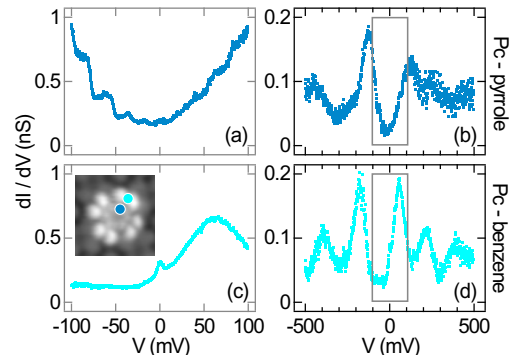
FIG. 2. Spectra of dI/dV acquired atop (a),(b) a pyrrole and (c),(d) a benzene moiety of Pc on graphene-covered Ir(111). Inset to (c): STM image (1 V, 10 pA, 2.5 nm \times 2.5 nm) of Pc embedded in a 2H-Pc island with marked (dots) positions of spectroscopy. Rectangles in (b),(d) mark the region of spectroscopic data in (a),(c). Feedback loop parameters: (a),(c) 0.1 V; (b),(d) 0.5 V and 50 pA.
