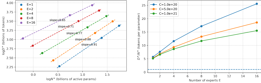
(a) Per- E cross-budget fits: D^* vs. N^* (b) Tokens-to-parameters drift across E (per budget)
