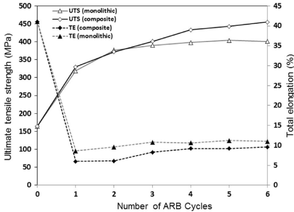
Fig. 8. UTS and TE values of the monolithic Cu and Cu/B 4 C composite materials.
