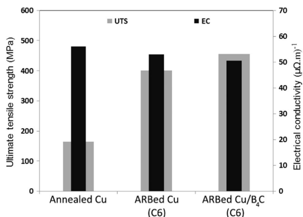
Fig. 12. UTS and EC comparison of the annealed monolithic Cu and six cycles ARB processed monolithic and Cu/B 4 C composite materials.
