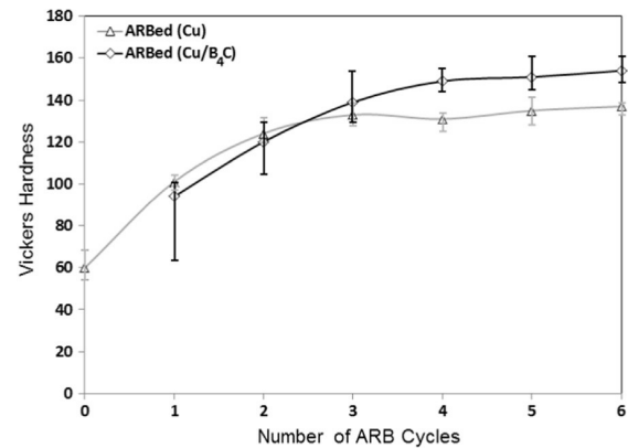
Fig. 7. Vickers microhardness of the monolithic and composite materials processed at different ARB cycles.
