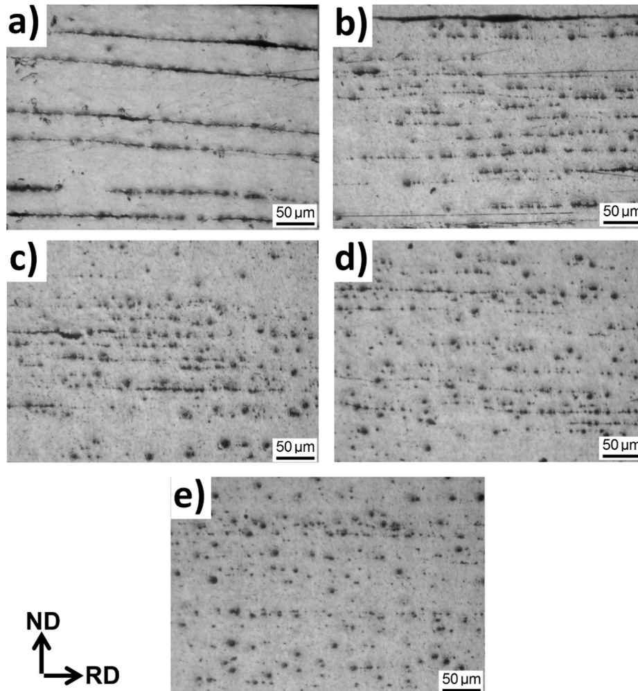
Fig. 2. OM micrographs of the composite samples processed to (a) two, (b) three, (c) four, (d) five and (e) six ARB cycles.
