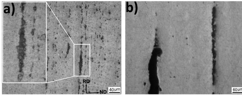
Fig. 3. High-magnification OM images of the Cu/B 4 C composites processed to (a) four and (b) two ARB cycles.
