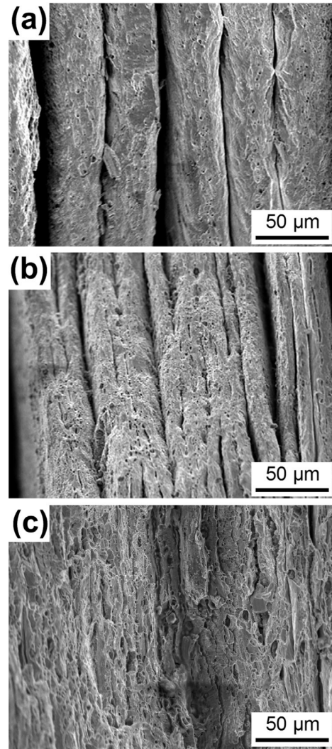
Fig. 9. Fracture surfaces of the composites: (a) C2, (b) C4 and (c) C6.
