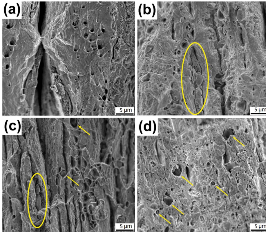
Fig. 10. High magnification SEM fractographs of the (a) two, (b) four, (c) five and (d) six cycles ARB processed Cu/B 4 C composites. The arrows show particles in the core of dimples as crack initiation sites; also, the ovals indicate particle agglomerated zones.
