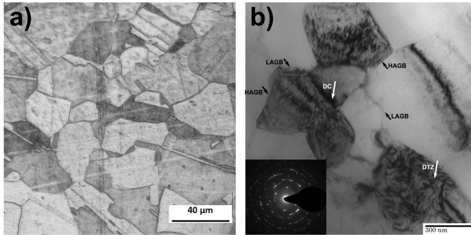
Fig. 6. (a) OM micrograph of the annealed Cu and (b) TEM microstructure of C6 matrix with the corresponding SAD pattern. High-angle grain boundaries (HAGBs) and low-angle grain boundaries (LAGBs), dislocation cell (DC), and dislocation tangle zones (DTZ) are shown in the TEM micrograph.
