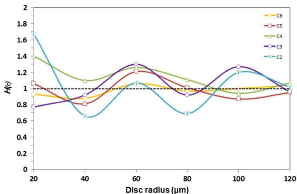
Fig. 4. Radial distribution function plots of the Cu/B 4 C composites fabricated from two to six ARB cycles, as nominated C2 to C6.
