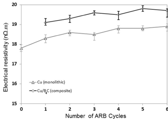
Fig. 11. ER of the ARBed monolithic and composite materials at different cycles.
