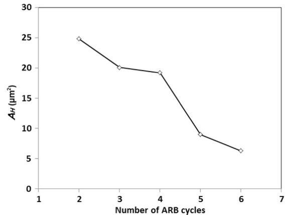
Fig. 5. Degree of clustering of the processed composites.
