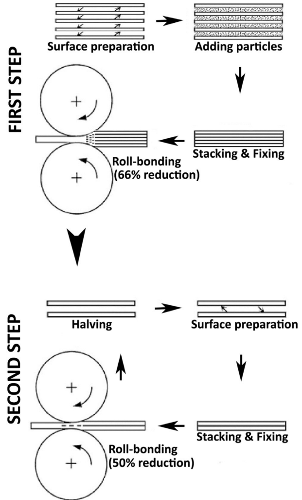
Fig. 1. Schematic illustration of the Cu/ B_4C composite production via the ARB process.
