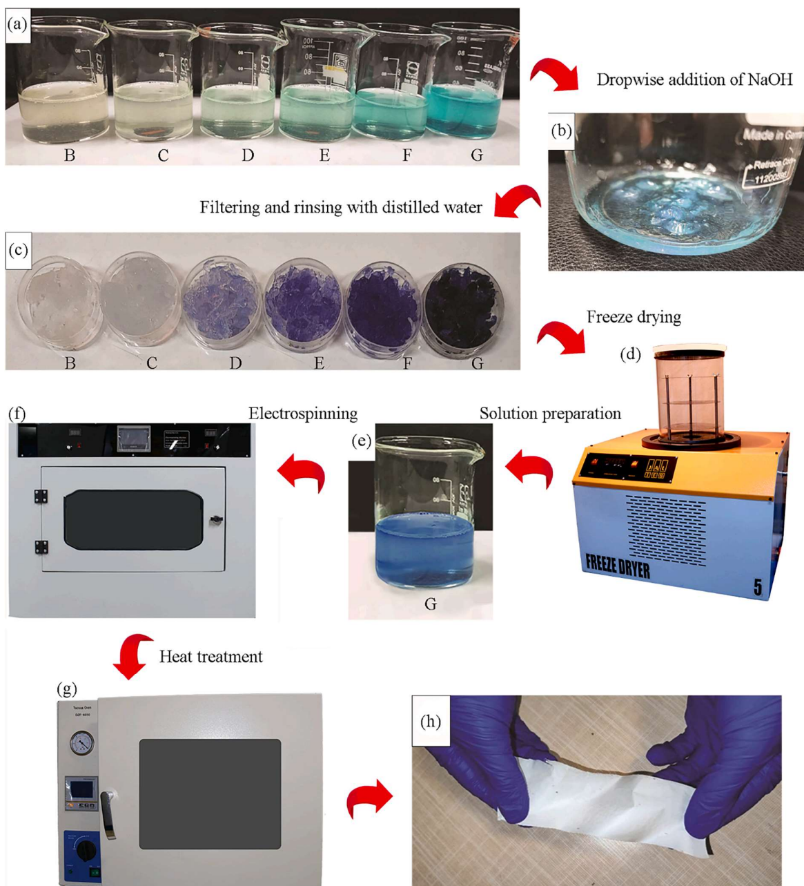
Fig. 1. Fabrication of chitosan-copper complexes/PVA electrospun mats: Chitosan solutions with the varying amounts of Cu (Table 1) (a), precipitation of chitosan-copper complexes by the dropwise addition of NaOH (b), collection of precipitants after rinsing with distilled water (c), obtaining chitosan-copper complex powders by freeze drying (d), preparation of electrospinning solutions by mixing chitosan-copper complexes solutions and PVA solutions in 30/70 ratio (e), electrospinning the mixed solution (f), crosslinking the detached mats by heat treatment (h), and final mats ready for further characterization (e).
