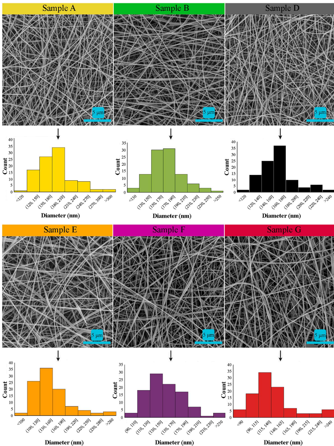
Fig. 3. Impact of the copper amount on the morphology and diameter distributions of the electrospun fibers.
