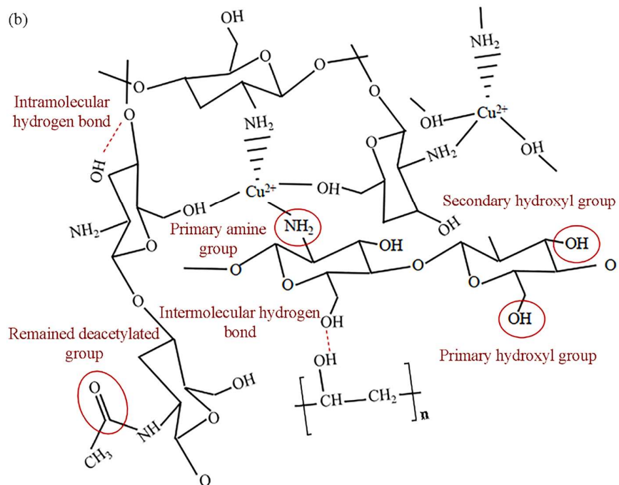
Fig. 4. FTIR spectra of the selected samples (a) and FTIR-derived structure of the chitosan-copper complex/PVA nanofibrous mats (b).
