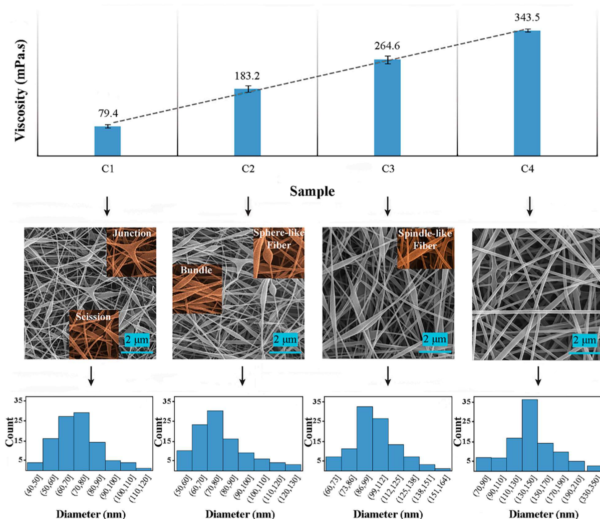
Fig. 2. Influence of the solution concentration and viscosity on the nanofiber morphology and diameter distribution.
