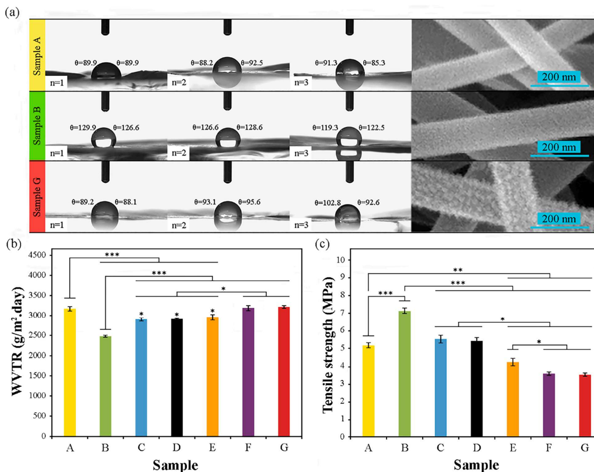
Fig. 5. Images of water droplets on selected mats, involving chitosan/PVA and chitosan complexed with the low and high copper amounts/PVA (a), WVTR of the electrospun mats (b), and effect of the amount of copper on the tensile strength of the wound dressings (c), with *, **, and *** denoting statistically significant differences with p < 0.05 , p < 0.01 , and p < 0.001 , respectively.
