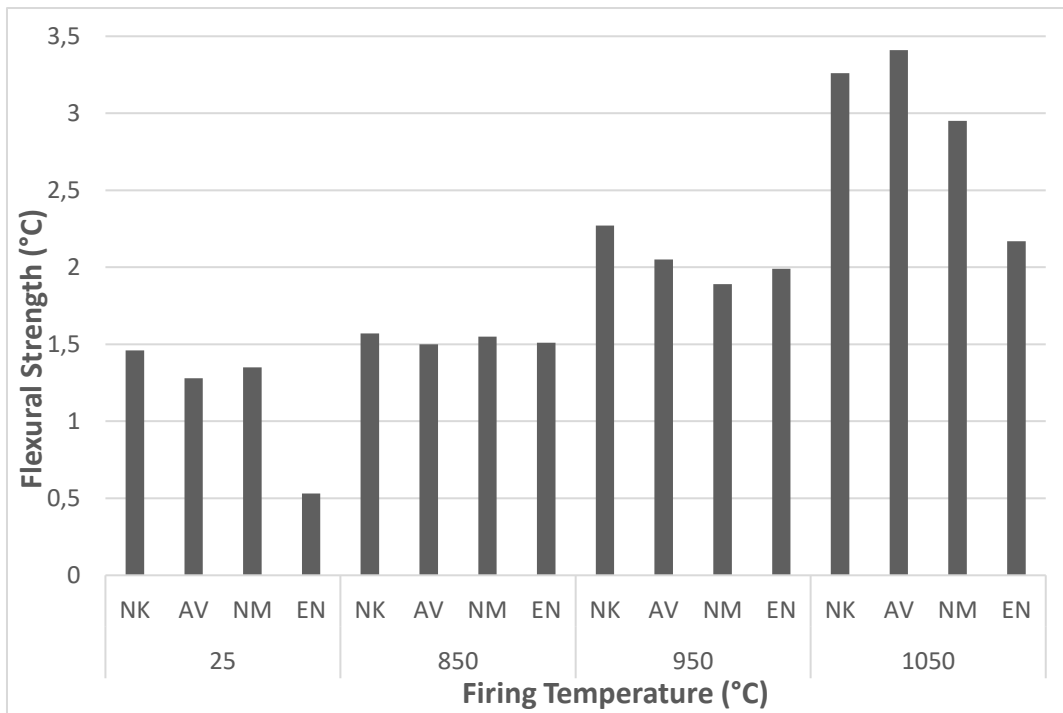
Figure 15: Flexural strength
