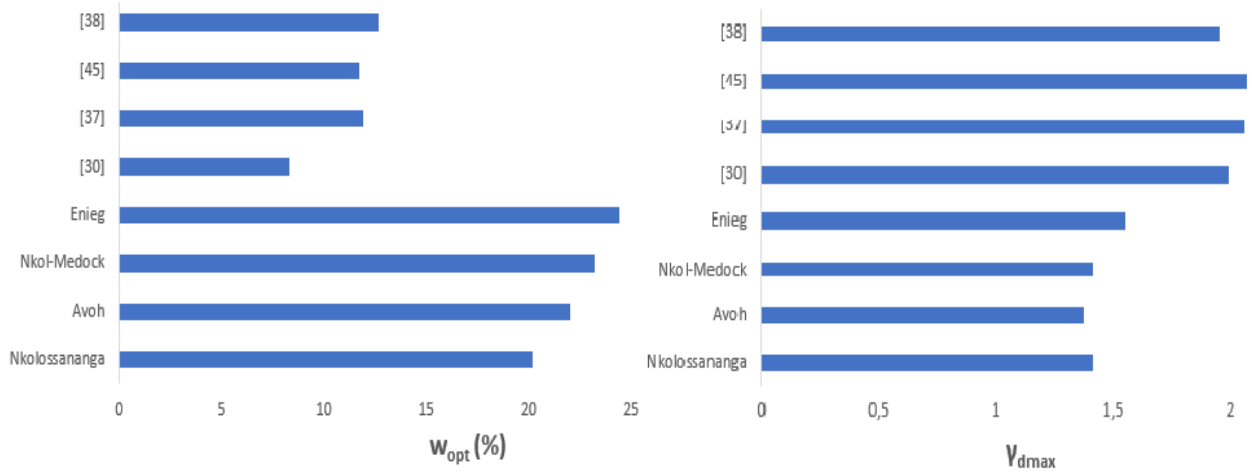
Figure 10: Comparison of the compaction parameters ( w_{opt} and \gamma_{dmax} ) with those of other authors
