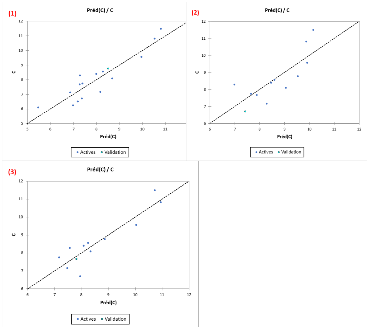
Figure 17: Measured values versus predicted values; 1: linear modeling between compressive strength and flexural strength; 2: linear modeling between compressive strength, absorption rate, density, and temperature; 3: Non-linear modeling between compressive strength, absorption rate, density, and temperature.
