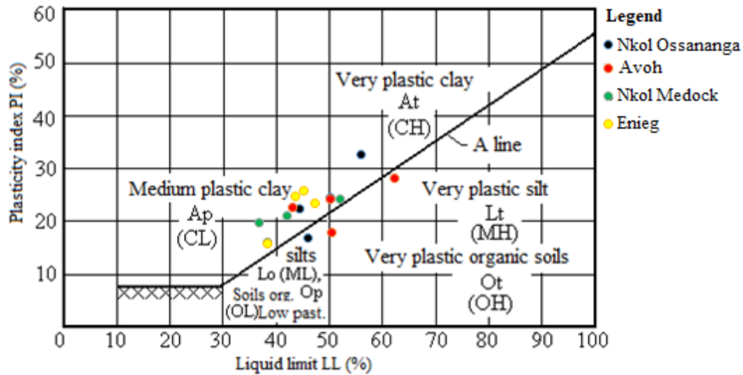
Figure 11: Casagrande plasticity diagram
