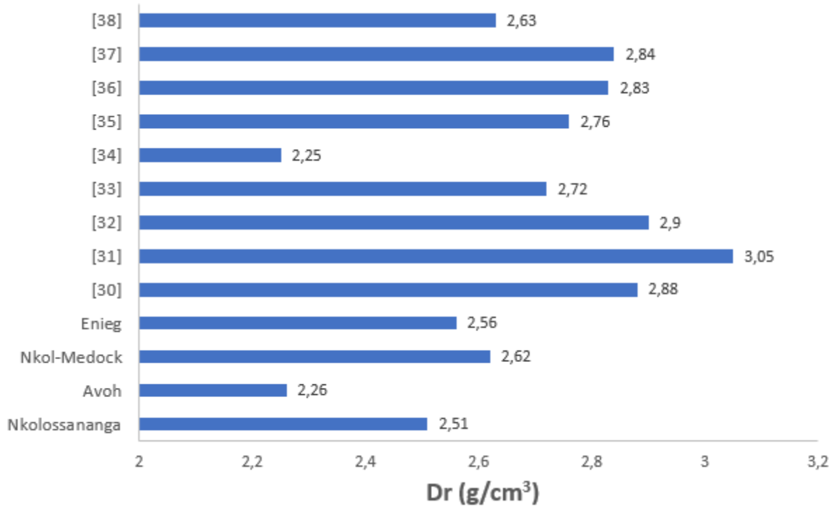
Figure 5: Comparison of specific gravity (Dr) values with those of other authors in previous works.
