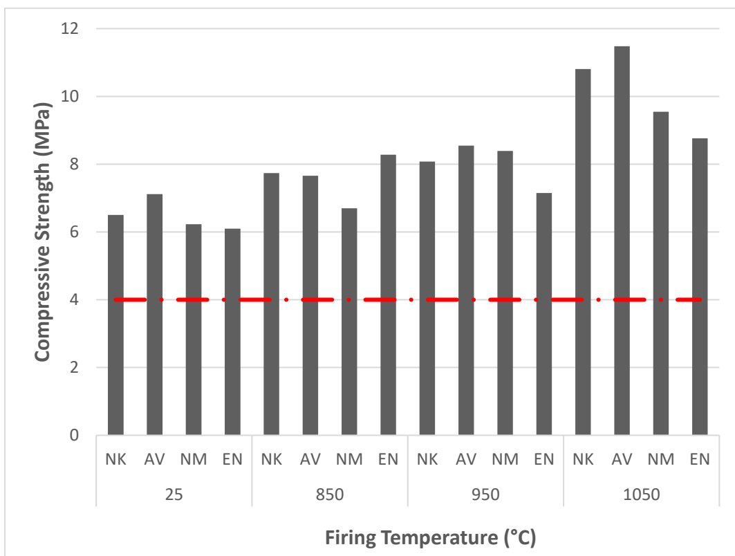
Figure 16: Compressive strength
