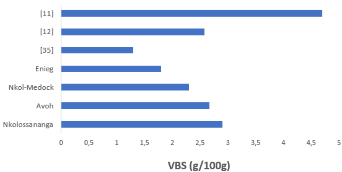
Figure 8: Comparison of the methylene blue values (VBS) with those of other authors
