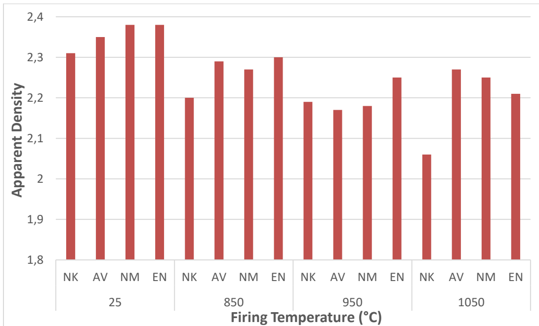
Figure 14: Apparent density of CEBs
