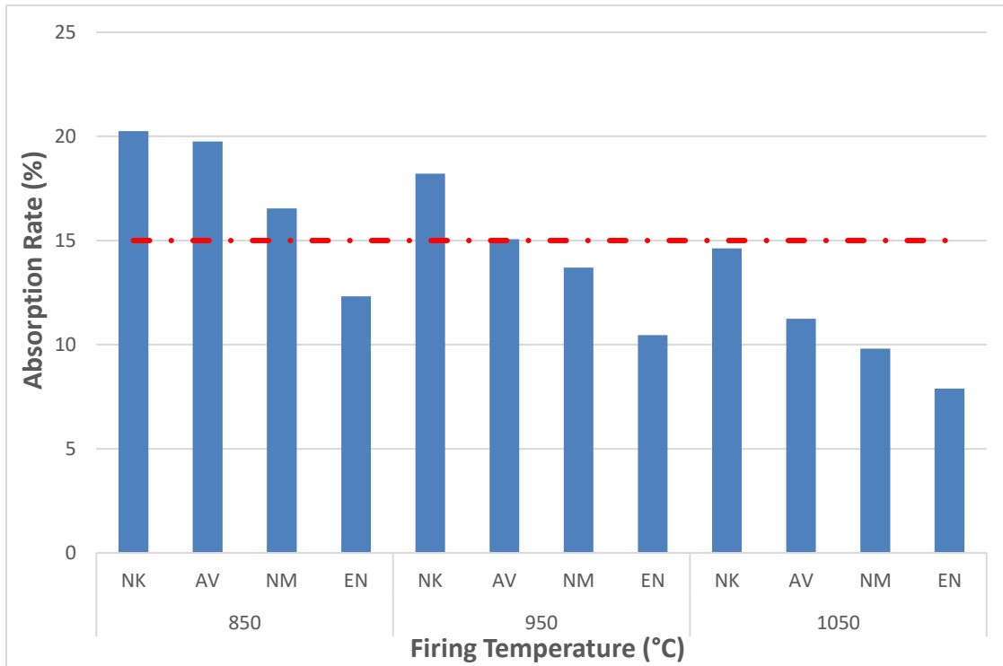
Figure 13: Water absorption of fired samples
