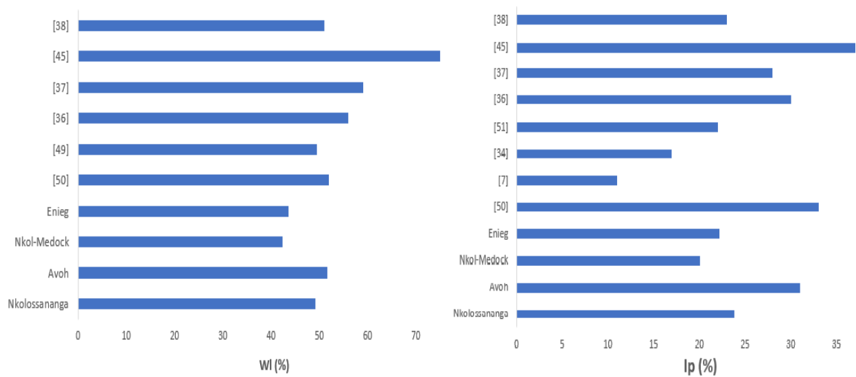
Figure 12: Plasticity (Wl and IP) of soils from other research works
