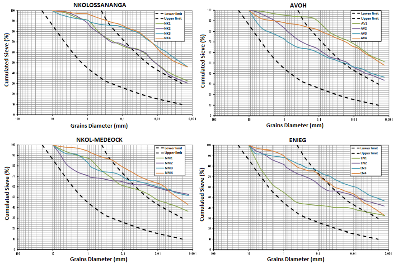
Figure 6: Grains size distribution
