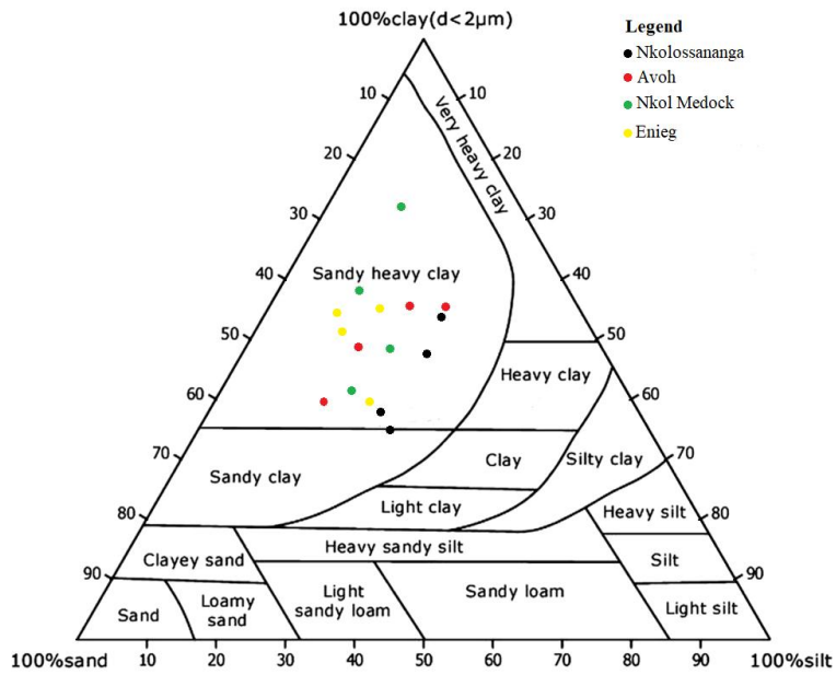
Figure 7: Ternary diagram from the Belgian classification
