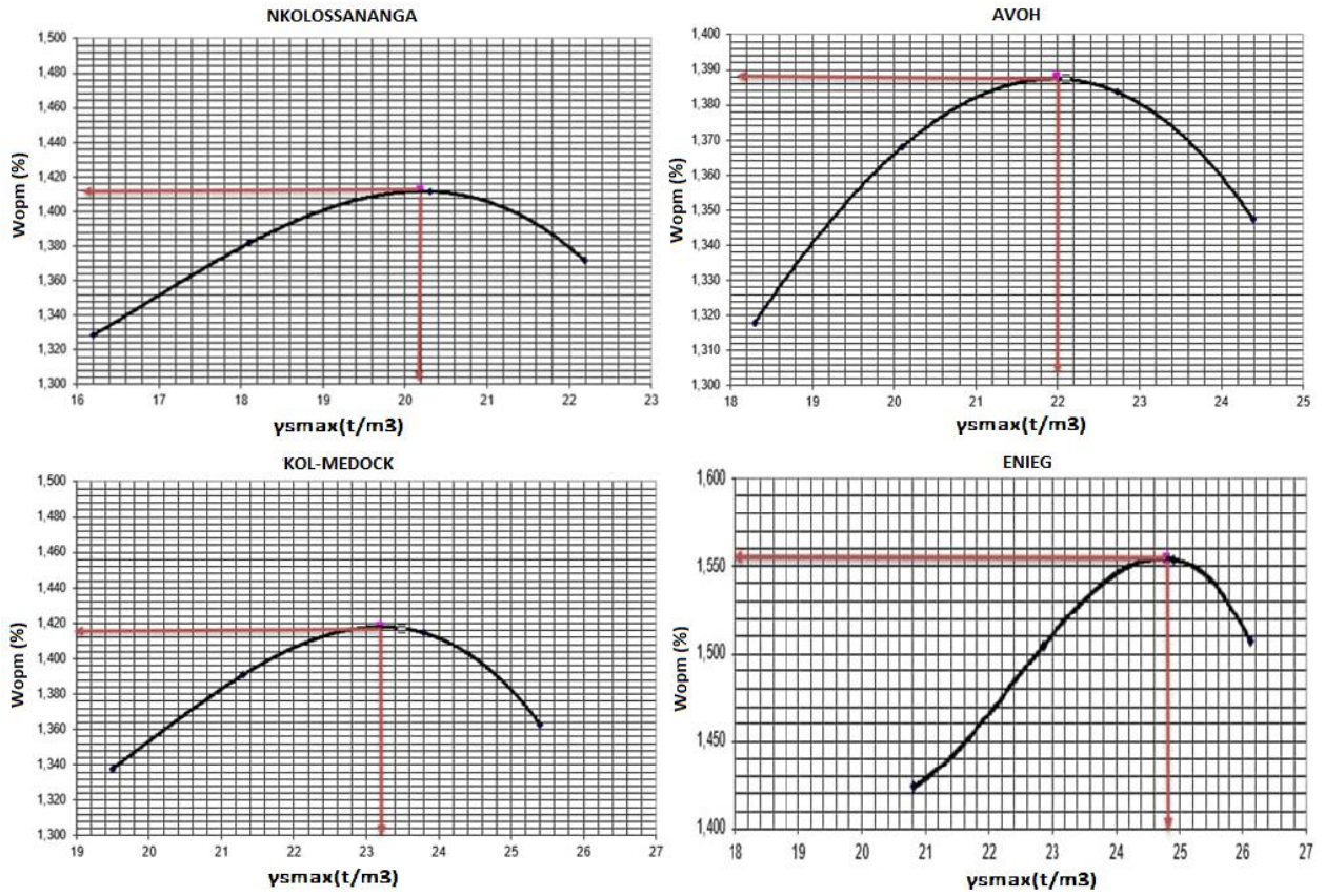
Figure 9: Proctor curves
